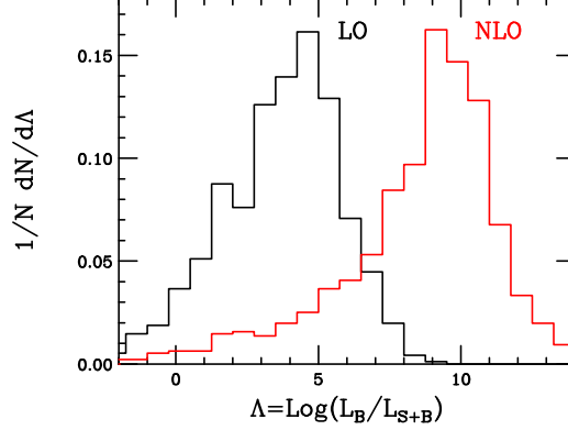
Figure 2: Pseudo experiments testing the hypothesis that there is a Higgs boson with m_H = 200 GeV. We generate pseudo-experiments which consist only of background and no Higgs signal. As such the most common outcome is that the signal plus background hypothesis is less likely than the background only.
