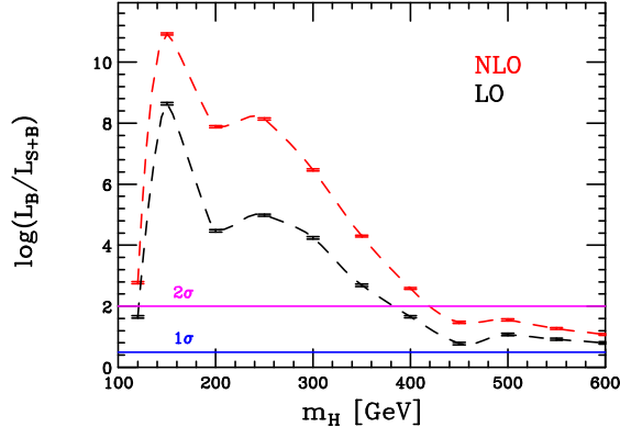
Figure 1: The log-likelihood difference for background only and signal plus background, for a Higgs boson search in the channel, H \rightarrow ZZ^* \rightarrow 4 leptons. Positive values of the difference indicate that the background-only hypothesis is more likely than the signal plus background one. The blue and magenta lines represent the 1- and 2- \sigma limits respectively.
