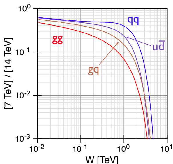
Fig. 2. Ratios of parton luminosities in pp collisions at \sqrt{s} = 7 TeV and 14 TeV. At W = 1 TeV, the curves from top to bottom refer to qq , u\bar{d} , gq , and gg , where q is a light ( u or d ) quark. The CTEQ6L1 parton distributions are used. (From Ref. [15].)
