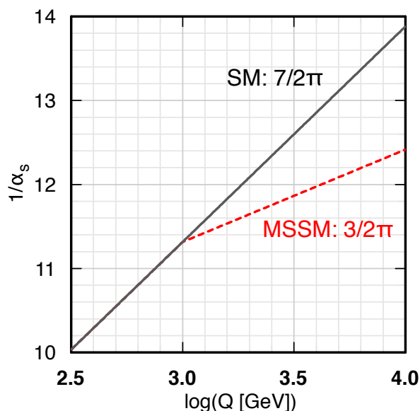
Fig. 1. Evolution of the strong coupling constant (displayed as 1/\alpha_s ) in the standard and supersymmetric versions of the SU(5) unified theory, for superpartners that become active at Q = 1 TeV.
