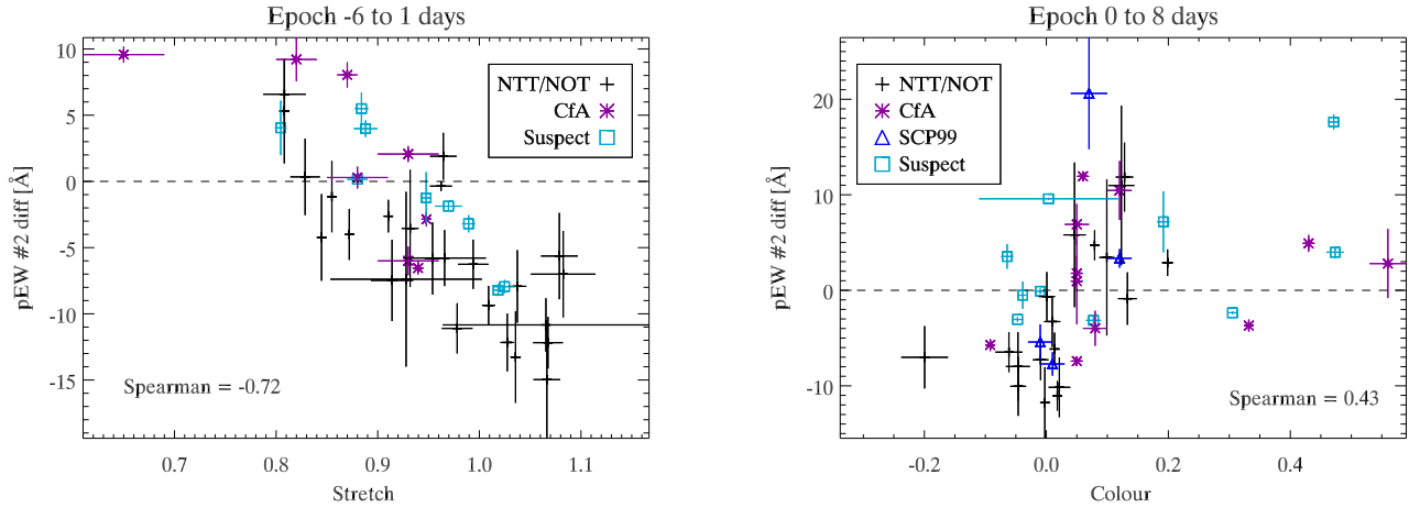
Fig. 12. These correlation studies show \Delta pEW , the measured pEW minus the expected pEW for the corresponding epoch (for the full sample of normal SNe Ia), vs SALT lightcurve parameter (stretch, colour) for different epoch intervals. These are given above each panel. The Spearman correlation coefficient is given in each plot. MC simulations show that the chance that these correlations are random consequences of a search through epoch ranges is one or less in 1000.
