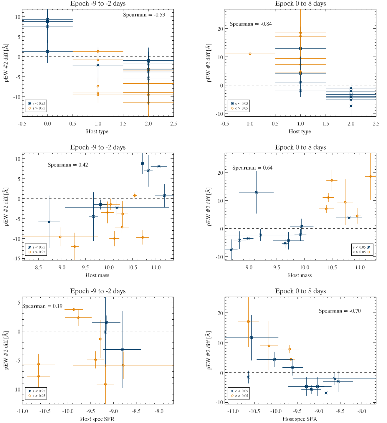
Fig. 14. Pseudo equivalent width of feature 2 compared with host galaxy properties. Left panels: Pre peak epochs (-9 to 2) with colours marking low/high lightcurve stretch SNe. Right panels: Post peak epochs (0 to 8) with colours marking low/high lightcurve colour SNe. Top: Host type vs pEW (0 not star forming, 1 moderately star forming, 2 highly star forming). Middle: Log of Host galaxy mass ( M_{\odot} ) vs. pEW. Bottom: Log specific star formation rate (log sSFR, \text{yr}^{-1} ) vs pEW.
