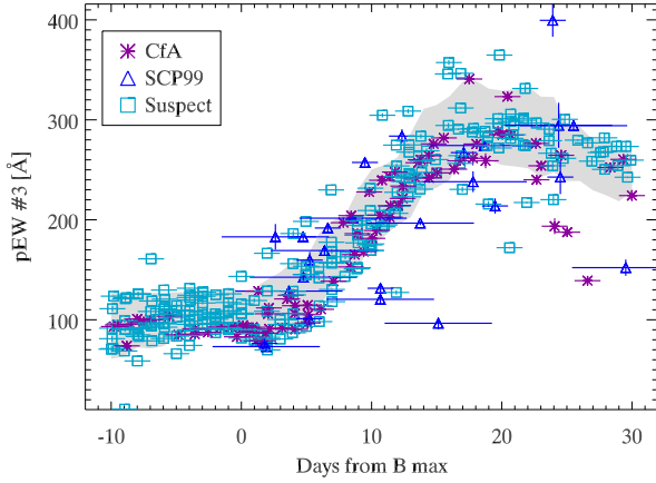
Fig. 6. pEW values for the reference data for f3 vs epoch. The shaded region is the same one sigma contour as shown in the left panel of Figure 8. The different symbols show the measurements that were used to construct the grey region, with different symbols denoting the different subsets of the reference sample.
