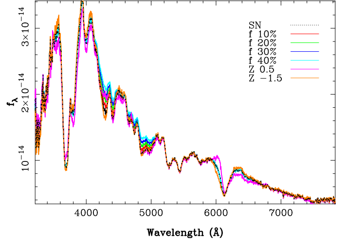
Fig. A.2. Models of evolution/metallicity changes applied to SN2003du. f (frac) models consist of a decrease in the depth of the f3 and f4 features, Z 0.5 corresponds to the Lentz et al. (2000) model of increased metallicity, Z -1.5 corresponds to the Lentz et al. (2000) model of decreased metallicity.
