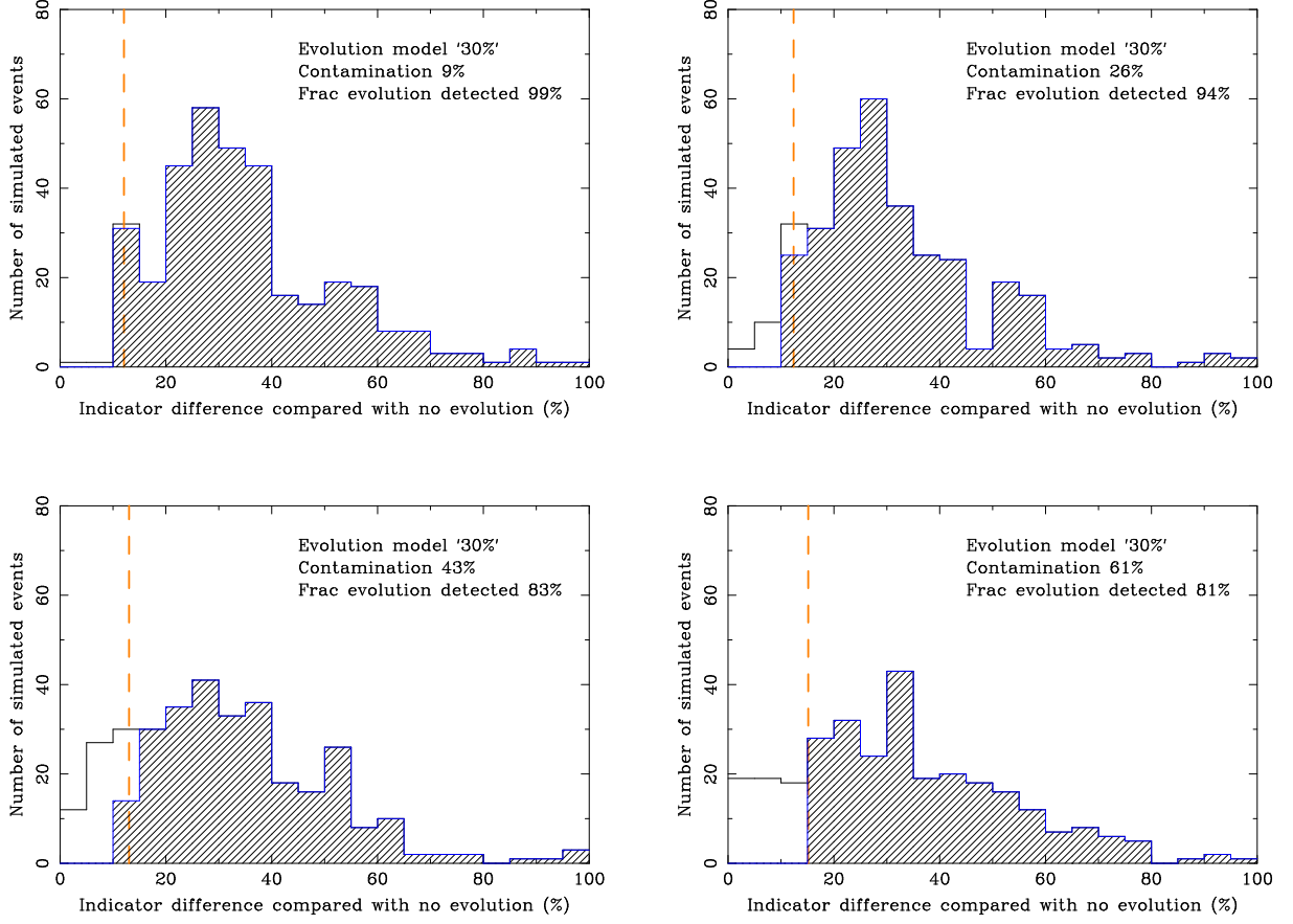
Fig. A.3. Sample study of how well evolution is detected in simulated spectra. The “30 %” evolution model was applied to all template spectra and the measured indicators compared with the unevolved measurements. The panels show the distribution of fractional difference, divided into the same contamination bins as in Figure A.1. The total uncertainty in each bin (bias and dispersion) as estimated above is shown as an orange dashed line. Events where the reported difference is larger than uncertainties would be seen as deviating. In this sense detectable events are shown as hashed bins. The fraction of detected events is shown in each panel. This fraction decreases with contamination.
