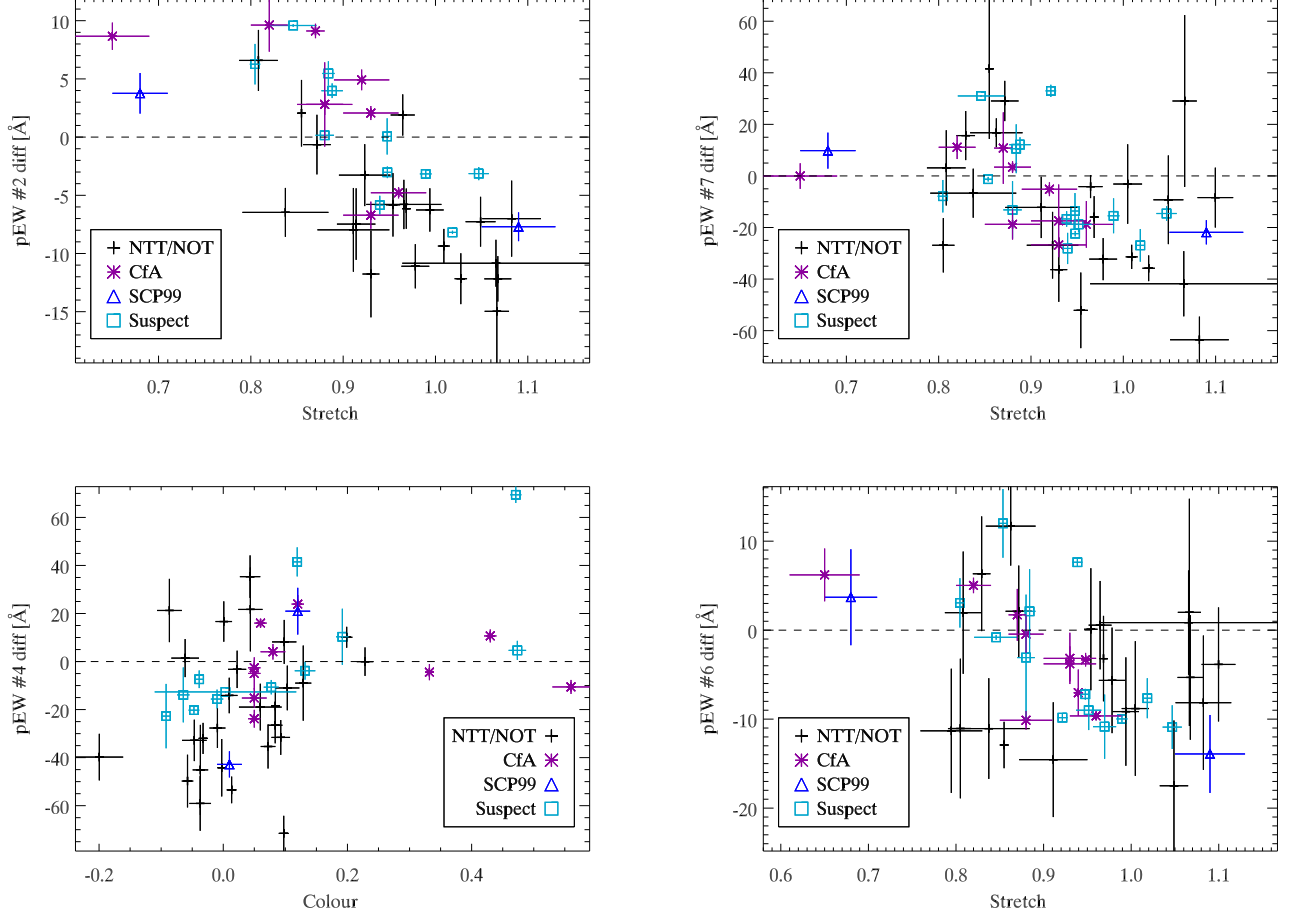
Fig. 11. These correlation studies show the measured pEW minus the expected pEW for the corresponding epoch for the full sample of normal SNe Ia vs SALT lightcurve parameter (stretch, colour) for epoch ranges around peak ( \pm 3 days). Indicators chosen are the ones showing largest correlation for this epoch range.
