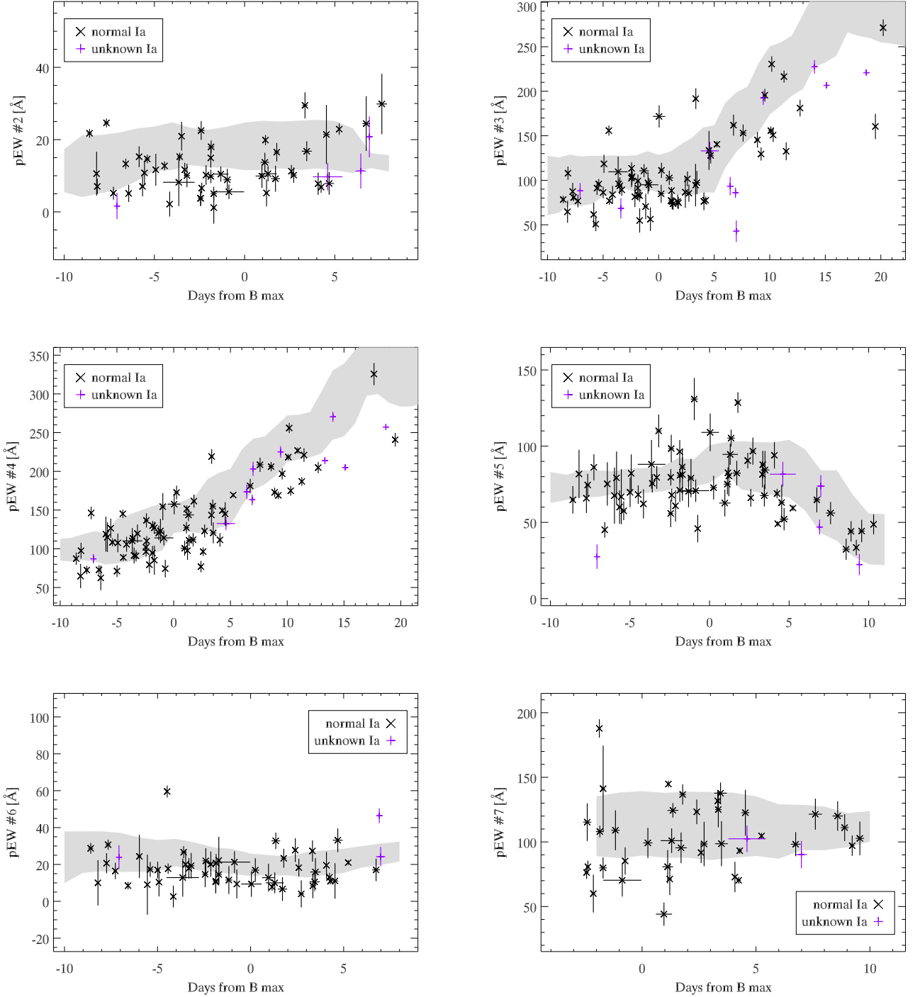
Fig. 8. Study of pseudo-equivalent widths for feature 2 to 7 vs epoch. The shaded band shows the one sigma contour for the normal SNe Ia in the reference sample. The points show the measurements on the NTT/NOT spectra, where the error bars include both statistical and systematic errors. The different symbols show two categories: spectra identified as of the normal SNe Ia subtype by SNID (SuperNova IDentification; Blondin & Tonry 2007) or spectra identified as SNe Ia but of unknown subtype.
