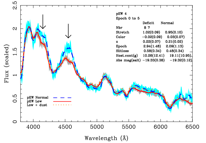
Fig. 18. Post peak, f4 deficit vs normal: Composite spectra of “reference normal” SNe (dashed blue) compared with pEW-deficit SNe (solid red) in the epoch range 0 to 5 days past peak brightness. The shaded regions correspond to jackknife dispersion (light blue for normal, grey for deficit). The dotted orange line corresponds to the deficit composite with Cardelli et al. (1989) dust applied matching the colour difference. The arrows indicate features commented on in the text. Mean properties of the composites are stated in Figure.
