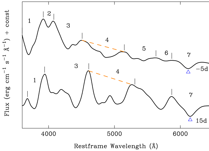
Fig. 1. The feature regions used for the measurements of spectral indicators are shown for two template spectra at day -5 and 15 relative to lightcurve peak (templates from Hsiao et al. 2007). The pseudo continuum (dashed orange) and line minimum (marked with blue triangle) are shown for two features (feature 4 and 7, respectively).
