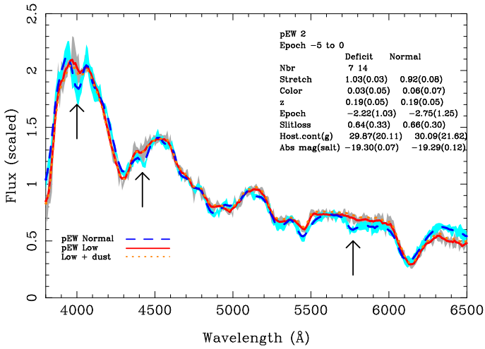
Fig. 17. Pre peak, f2 deficit vs normal: Composite spectra of “reference normal” SNe (dashed blue) compared with pEW-deficit SNe (solid red) in the epoch range -5 to 0 days past peak brightness. The shaded regions correspond to jackknife dispersion (light blue for normal, grey for deficit). The dotted orange line corresponds to the deficit composite with Cardelli et al. (1989) dust applied that matches the colour difference. The arrows indicate features discussed in the text. Mean properties of the composites are stated in the Figure.
