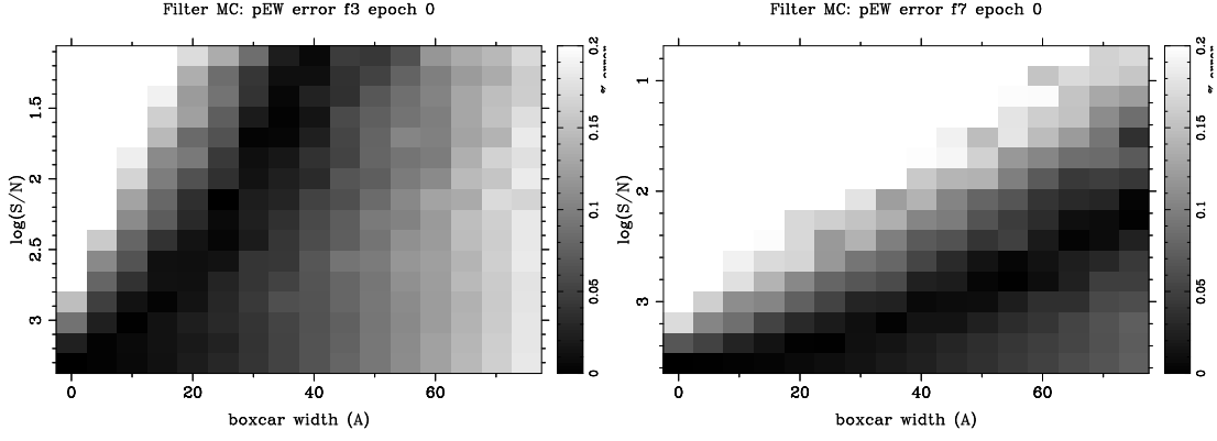
Fig. B.1. Average pEW error for feature 3 (left panel) and feature 7 (right panel) at the epoch of maximum light. The noise level, expressed through the logarithm of the pseudo-S/N, increases along the y-axis and the filter strength along the x-axis. Darker shades show smaller errors.
