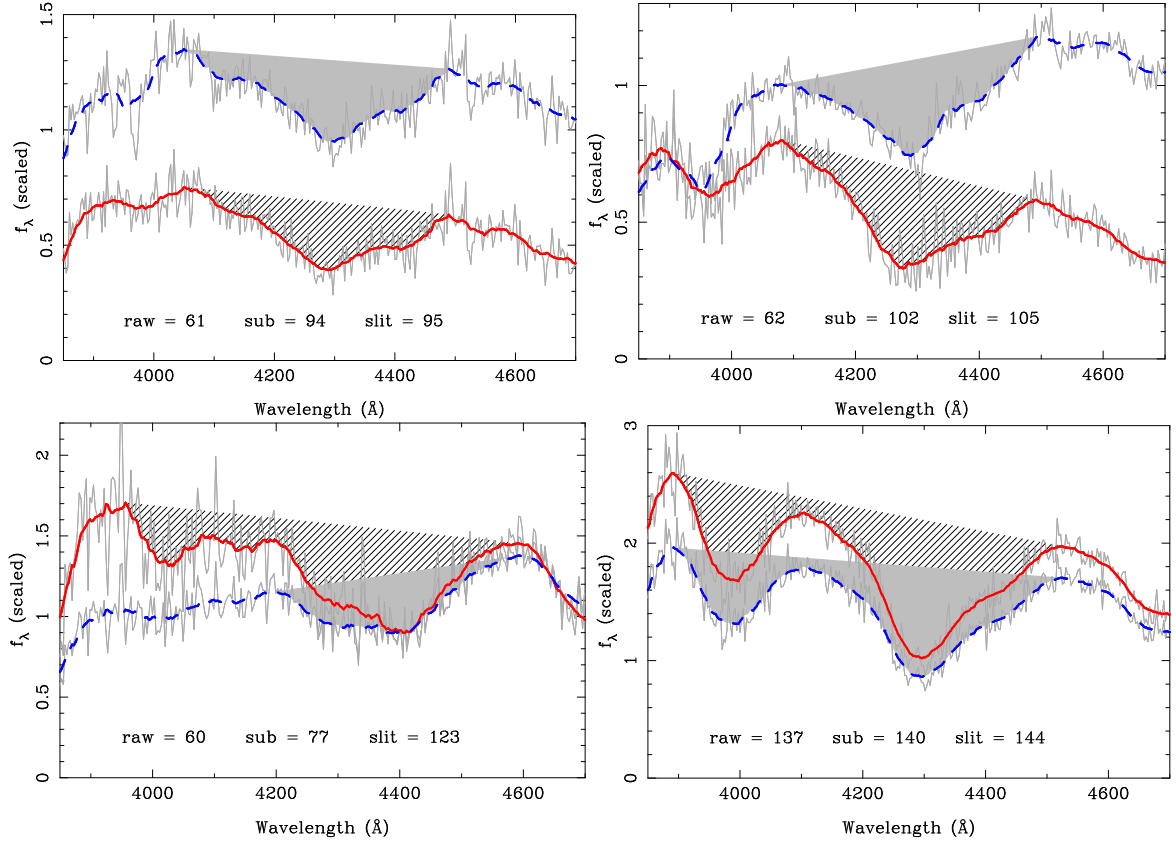
Fig. 5. Expanded view of the feature 3 region for the same spectra displayed in Figure 4, showing the effects of host subtraction and slit loss/reddening correction on pEW. Wavelength (x-axis) is rest-frame wavelength. The blue dashed line is the raw spectrum, the red solid line the final subtracted and corrected spectrum. The marked regions show where pEW is calculated, the calculated pEWs (in Å) are written in panels for raw spectra (“raw”), subtracted spectra (“sub”) as well as subtracted and corrected spectra (“slit”). These sample spectra show host subtraction change pEWs both through additive offsets and changed feature limits.
