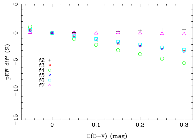
Fig. 2. Percent change in pEW for features 2 to 7 as a function of E(B - V) . The measurements are based on the Hsiao et al. (2007) SN template at peak brightness and assuming Cardelli et al. (1989) type dust with R_V = 1.7 .
