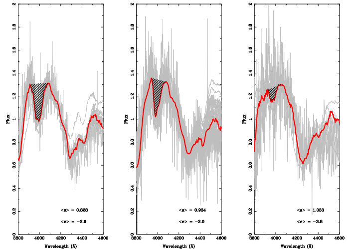
Fig. 15. Composite spectra constructed from all peak spectra (NTT/NOT as well as reference SNe), divided according to stretch. The average lightcurve stretch, s , is printed in each panel, increasing from left to right. The average epoch, e , is also included for each composite. The plots show both the composite (thick red) and individual (grey) spectra.
