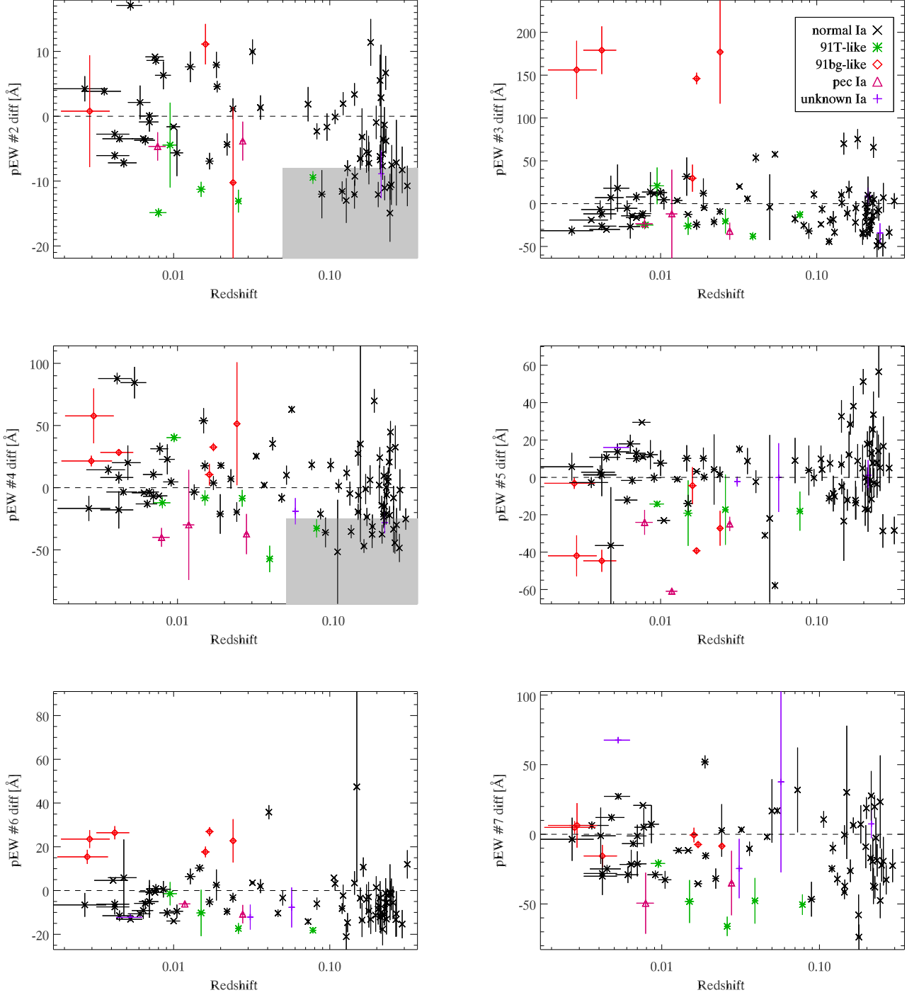
Fig. 9. Comparison of the pseudo-equivalent width measurements around lightcurve peak for features 2 to 7 vs redshift. In all figures the average spectroscopic evolution among non-peculiar low-z reference SNe has been subtracted. It is thus the pEW-difference (compared to normal low-z SNe) that is plotted on the y-axis. SNe are divided according to subtype classification, with the colour scheme following the legend in the upper right plot. In the two upper left panels (f2 and f4) the shaded region show how the pEW-deficit sample is defined.
