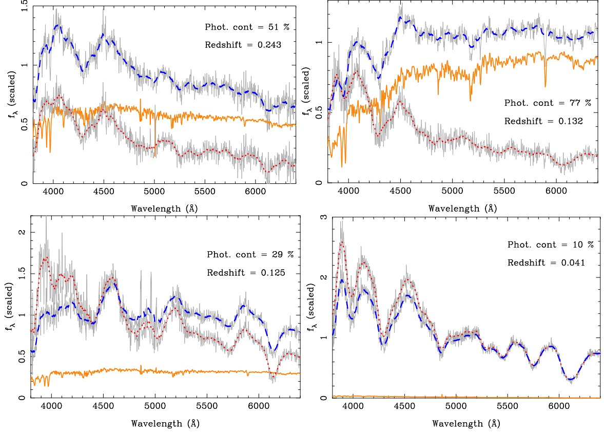
Fig. 4. Display of sample host galaxy subtractions of SDSS SN16637, 12907, 17886 and 13894 (clockwise from top left, restframe epochs -1, 0, -4 and 9). All flux values (y-axis) have been scaled. Wavelength (x-axis) is rest-frame wavelength. The grey line shows the unsmoothed original spectrum, while the dashed blue line shows the smoothed version. Dotted red line show final subtracted slit loss/reddening corrected spectrum and orange solid line show best fit galaxy. Note that because of the slit loss/reddening correction the galaxy and subtracted spectrum do not sum to the raw spectrum. The galaxy contamination estimated from photometry (g-band) and redshift have been written in each panel.
