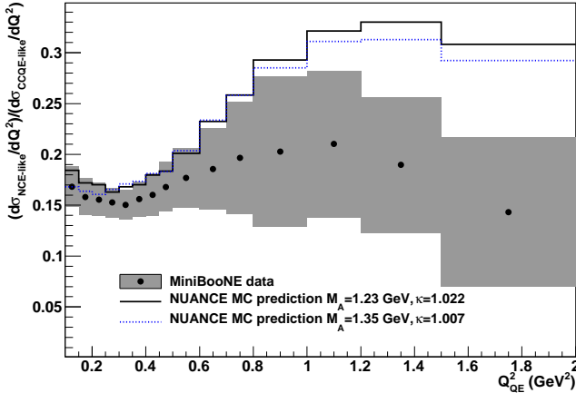
FIG. 7: MiniBooNE NCE-like/CCQE-like cross-section ratio on \text{CH}_2 as a function of Q_{QE}^2 with total error. The color code for the histograms is the same as in Figure 6.
