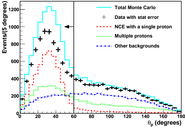
FIG. 11: The angle between the reconstructed nucleon direction and the incident beam direction for data and MC after the NCE, “Proton/Muon”, and “Proton/Neutron” cuts. All distributions are POT-normalized. Events with \theta_p < 60^\circ are used in the analysis.
