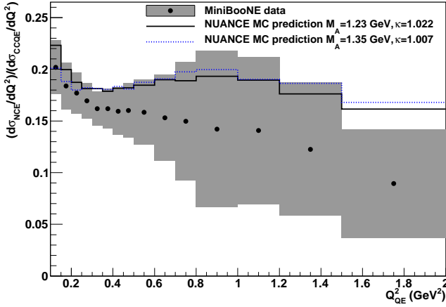
FIG. 6: MiniBooNE NCE/CCQE cross section ratio on \text{CH}_2 as a function of Q_{QE}^2 . The NUANCE MC prediction is plotted for two assumptions of parameters: black solid line for M_A = 1.23 GeV and \kappa = 1.022 [5], and blue dotted line for M_A = 1.35 GeV and \kappa = 1.007 [19]. \Delta s is assumed to be zero in both of these cases. Both cross sections in the ratio are per target nucleon – there are 14/6 times more target nucleons in the numerator than in the denominator. The error bars represent both statistical and all systematic uncertainties (excluding flux errors) taken in quadrature.
