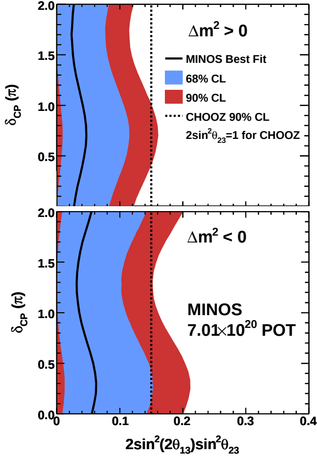
FIG. 4: Values of 2\sin^2(2\theta_{13})\sin^2\theta_{23} and \delta_{CP} that produce a number of candidate events in the Far Detector consistent with the observation for the normal hierarchy (top) and inverted hierarchy (bottom). Black lines show those values that best represent our data. Red (blue) regions show the 90% (68%) C.L. intervals. The CHOOZ limit is drawn for \Delta m_{32}^2 = 2.43 \times 10^{-3} \text{eV}^2 , \sin^2(2\theta_{23}) = 1.0
