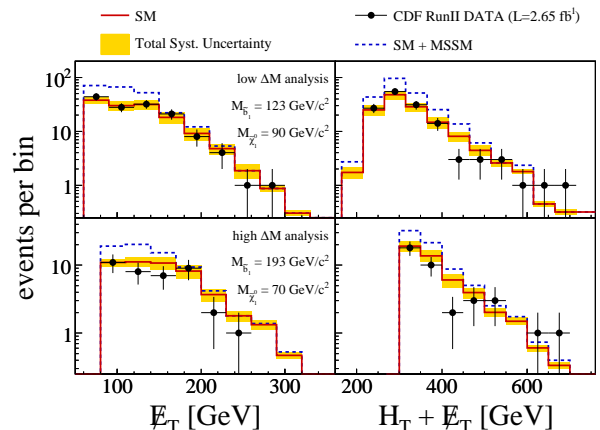
FIG. 1: Measured \cancel{E}_T and H_T + \cancel{E}_T distributions (black dots) for low- \Delta M (top) and high- \Delta M analyses (bottom), compared to the SM predictions (solid lines) and the SM+MSSM predictions (dashed lines). The shaded bands show the total systematic uncertainty on the SM predictions.
