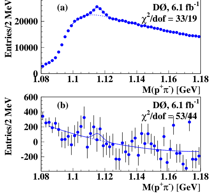
FIG. 27: The p\pi^- invariant mass distribution of \Lambda candidates in the inclusive muon sample for p \rightarrow \mu with 4.2 < p_T < 7.0 GeV. (a) The sum of distributions of positive and negative p \rightarrow \mu tracks and (b) their difference. The solid lines present the result of the fit and the dashed lines show the background contribution.
