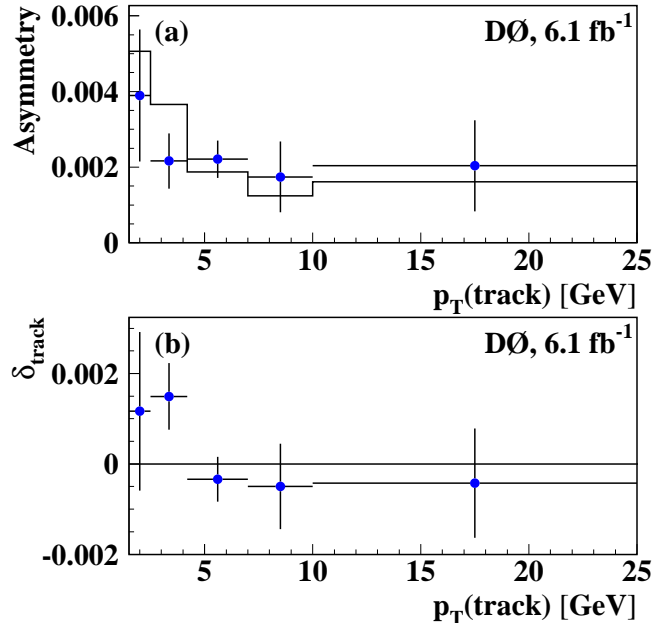
FIG. 28: (a) The expected (points with errors) and measured (histogram with negligible uncertainties) track reconstruction asymmetry. (b) The quantity \delta_{\text{track}} = a_{\text{track}} - a_K^{\text{track}} f_K^{\text{track}} .
