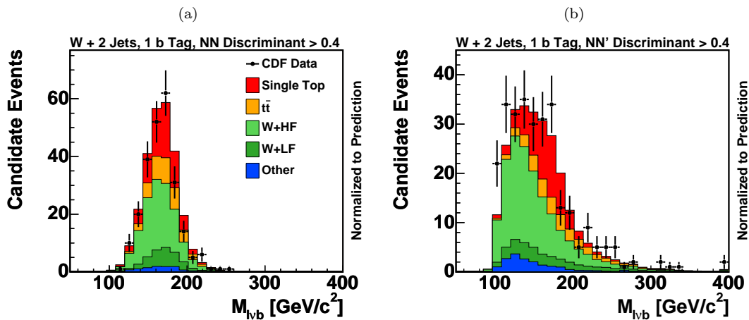
FIG. 29: Comparison of the predictions and the data for M_{l\nu b} for events with an output above 0.4 of the original NN (left) and a specially trained NN' (right) discriminant. The data are indicated by points with error bars, and the predictions are shown stacked, with the stacking order following that of the legend.
