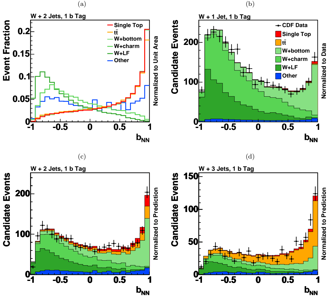
FIG. 14: Templates (a) of the jet flavor separator b_{NN} for W +light, W +charm (adding the Wc\bar{c} and Wcj contributions because of their similar shapes), and W +bottom events. The template labeled “Other” represents the diboson and Z/\gamma^* +jets contributions. The strong discrimination b_{NN} provides to separate jet flavors makes it a powerful variable in multivariate analyses. Panel (b) shows the outcome of the fit to the W +1 jet data sample allowing the b , c , and light-flavor components to float as described in Section V. Panels (c) and (d) compare the data and the corresponding predictions in the W +2 jet and W +3 jet samples. In panels (b) through (d), the data are indicated with points with error bars, and the model predictions are shown with shaded histograms, stacked in the same order as the legend.
