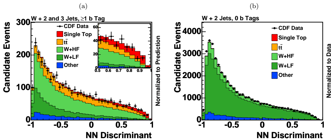
FIG. 28: Comparison of the data with the sum of the predictions of the neural network output for the sum of all selected signal data samples (left) and the neural network output for two-jet one- b -tag events applied to the untagged control sample, showing close modeling of the data and good control over the W +light-flavor shape. The data are indicated by points with error bars, and the predictions are shown stacked, with the stacking order following that of the legend.
