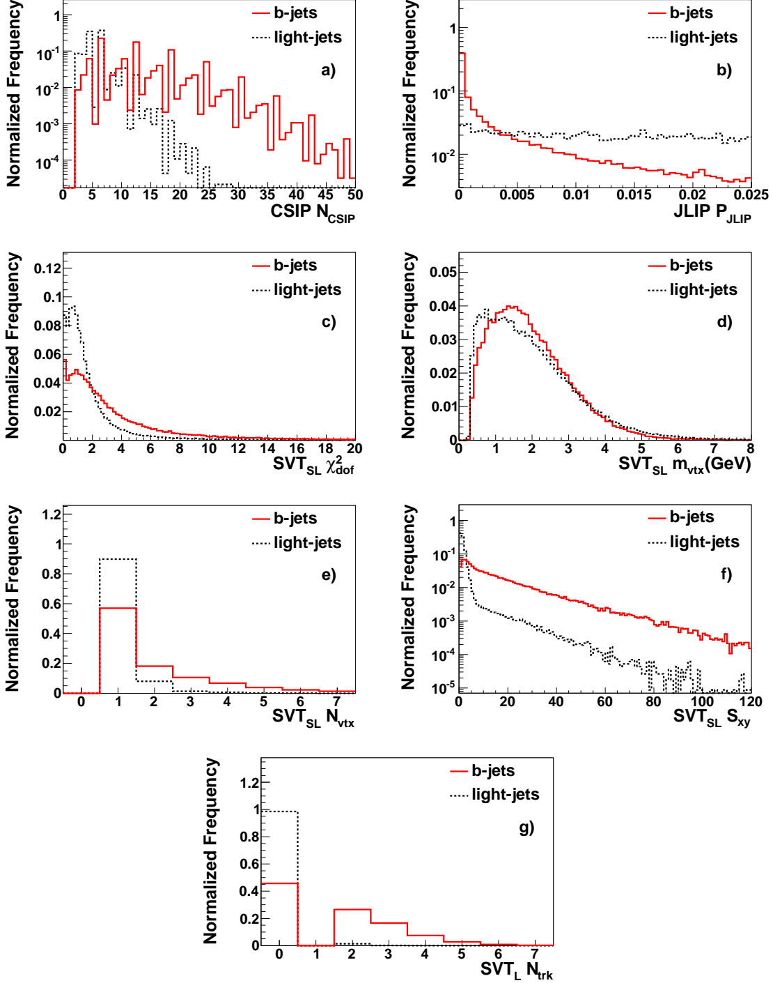
Figure 18: The NN variables \text{CSIP } \mathcal{N}_{\text{CSIP}} (a), \text{JLIP } \mathcal{P}_{\text{JLIP}} (b), \text{SVT}_{\text{SL}} \chi_{\text{dof}}^2 (c), m_{\text{vtx}} (d), N_{\text{vtx}} (e), S_{xy} (f), and \text{SVT}_L N_{\text{trk}} (g) for QCD b\bar{b} MC (continuous lines), and light jet QCD MC (dashed lines). All histograms are normalized to unit area.
