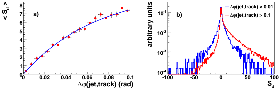
Figure 15: Mean signed impact parameter significance S_d (averaged over all tracks in all b -jets in simulated events) as a function of the azimuthal angle between the track and b -jet directions \Delta\phi (a) and S_d distributions for tracks at low and high \Delta\phi (b).
