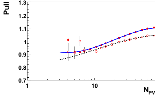
Figure 10: Fitted pull values of the track impact parameters, corrected here for their p_{\text{scat}} and category dependence, as a function of the number of tracks attached to the primary vertex, combining all track categories. The superimposed solid (dashed) curves are empirical parametrizations of the data (QCD MC).
