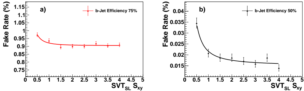
Figure 19: Fake rate for fixed signal efficiencies of 75% (a) and 50% (b) as a function of the SVT_{SL} \mathcal{S}_{xy} requirement on the input jets. The lines are intended to guide the eye only.
