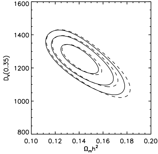
Figure A2. Comparison of the LRG-only likelihood surface computed with the analytic approximation of P_{nw} in Eqn. 29 of Eisenstein & Hu (1998) (solid, as in Fig. 5) compared with the result when using the b-spline fit described in Appendix A3 (dashed).
