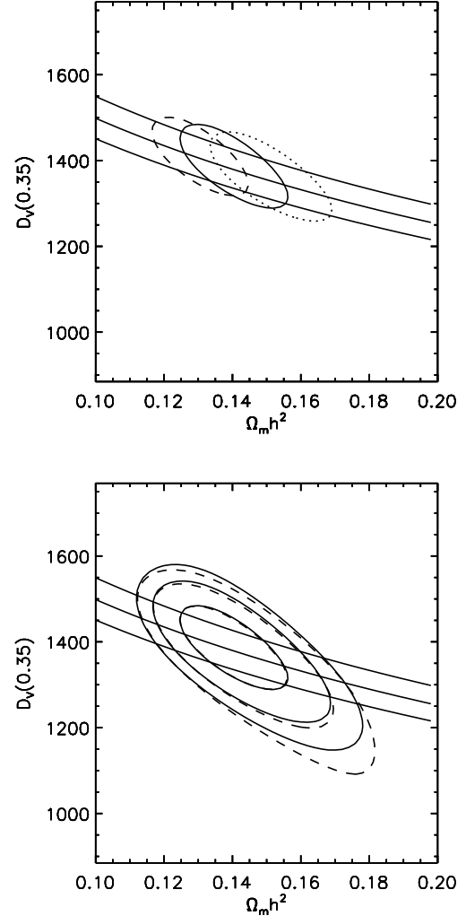
Figure 6. Upper panel: Change in \Delta\chi^2 = 2.3 contour as n_s is varied, with all other parameters as in Fig. 5. n_s = 1.02 (dashed), n_s = 0.96 (solid), and n_s = 0.90 (dotted). The degeneracy is well-described as \Omega_m h^2 (n_s/0.96)^{1.2} = 0.14 . Lower panel: The impact of assuming a \Lambda CDM relation between \Omega_m , h , and D_V (solid contours) compared with applying the non-linear corrections at h = 0.7 and assuming no relation between \Omega_m , h , and D_V(0.35) (dashed contours). As in Fig 5 the lines show the constraints for constant r_s/D_V(0.35) from P09.
