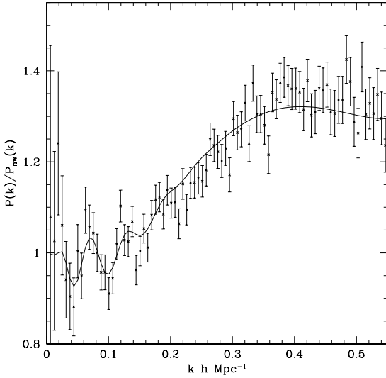
Figure B5. Agreement between P_{halo, WMAP3}(k)/P_{nw}(k, \mathbf{p}_{WMAP3}) measured from the catalogues in Reid & Spergel (2009) based on an N -body simulation z = 0.2 snapshot with WMAP3 cosmological parameters (points with error bars) vs. the model prediction from Eqn 16 at z_{NEAR} = 0.235 .
