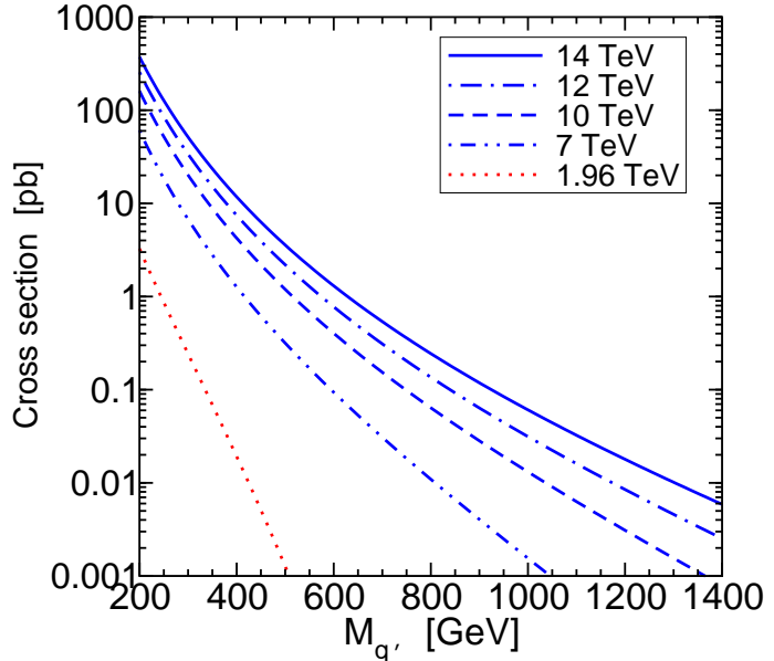
FIG. 11: Production cross-section for new quarks as a function of the mass, for the Tevatron p\bar{p} collisions at \sqrt{s} = 1.96 TeV, and for the LHC pp collisions with \sqrt{s} = 7, 10, 12 , and 14 TeV. The graph was made at leading order using CTEQ5LO parton distribution functions [53] with Q = m_{q'} and applying a K factor of 1.5 for LHC and 1.25 for Tevatron.
