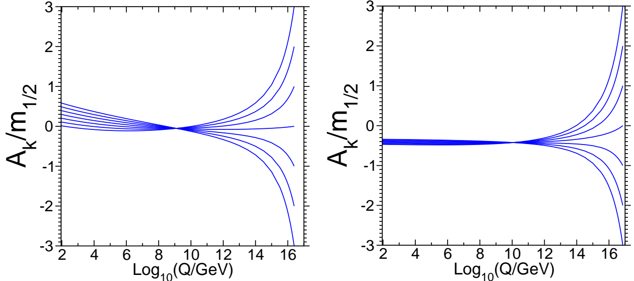
FIG. 5: Renormalization group running of scalar trilinear couplings A_{k_N} in the LND model (left panel) and A_{k_U} in the QUE model (right panel), normalized to m_{1/2} , the common gaugino mass parameter at the unification scale M_{\text{unif}} . The different lines correspond to different boundary conditions at M_{\text{unif}} . The corresponding Yukawa couplings k_N and k_U are taken to be near their fixed-point trajectories, with k_N = 3 and k_U = 3 at M_{\text{unif}} . The running of A_{k_D} in the QDEE model is very similar to that shown here for A_{k_U} .
