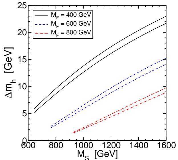
FIG. 8: Corrections to m_{h^0} in the QUE model with k_U = 1.05 , for varying m_{1/2} with other parameters described in the text. Here M_F = 400, 600, and 800 \text{ GeV} is the vector-like superpotential fermion mass term, and M_S is the geometric mean of the new up-type scalar masses. The upper and lower lines in each case correspond to A_k = -0.5m_{1/2} and A_k = -0.3m_{1/2} , respectively, at the TeV scale. The value of m_{h^0} before these corrections is assumed to be 110 GeV.
