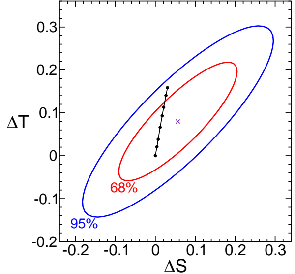
FIG. 10: Corrections to electroweak precision observables S, T from the QUE model at the fixed point (k_U, h_U) = (1.050, 0) , for varying M_Q = M_U = m_{b'} , with m_{1/2} = 600 GeV and A_{k_U} = -0.4m_{1/2} and m_0 = 0 and b_Q = b_U = -m_{1/2}M_Q , using eqs. (2.11) and (2.13). The eight dots on the line segment correspond to m_{t'_1} = 275, 300, 350, 400, 500, 700, 1000 GeV and \infty , from top to bottom. The experimental best fit is shown as the \times at (\Delta S, \Delta T) = (0.057, 0.080) . Also shown are the 68% and 95% CL ellipses, obtained as described in the text. The point \Delta S = \Delta T = 0 is defined to be the Standard Model prediction for m_t = 173.1 GeV and m_{h^0} = 115 GeV. Results for the QDEE model are very similar.
