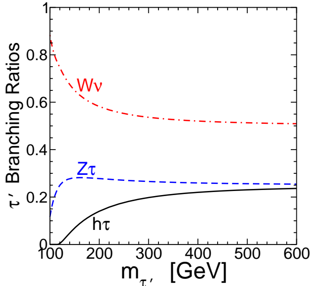
FIG. 14: Branching ratios for \tau' decays to W\nu , Z\tau , and h^0\tau in the QUE and QDEE models, as a function of m_{\tau'} .
