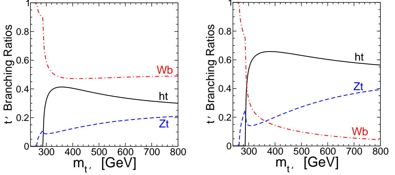
FIG. 13: Branching ratios for the lightest extra quark, t'_1 , in the QUE model with M_Q = M_U , to final states Wb , Zt , and h^0t , as a function of m_{t'_1} . The left panel shows the “democratic” case that arises when \epsilon_U dominates (with equal charged and neutral currents), and the right panel shows the “ W -phobic” (mostly neutral current) case that arises when \epsilon'_U dominates. In the “ W -philic” case that arises when \epsilon_D dominates, then BR(t' \rightarrow Wb) = 1 (not shown).
