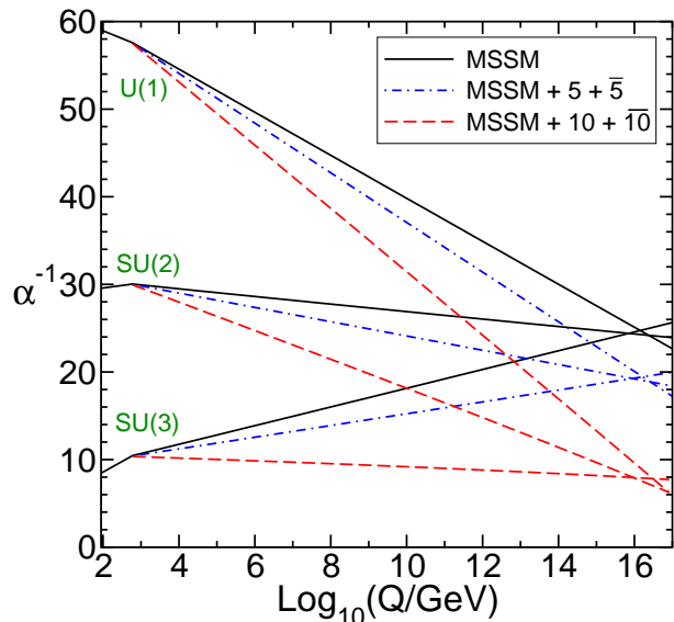
FIG. 1: Gauge coupling unification in the MSSM, LND and QUE models. The running is performed with 3-loop beta functions, with all particles beyond the Standard Model taken to decouple at Q = 600 GeV, and m_t = 173.1 GeV with \tan\beta = 10 .
