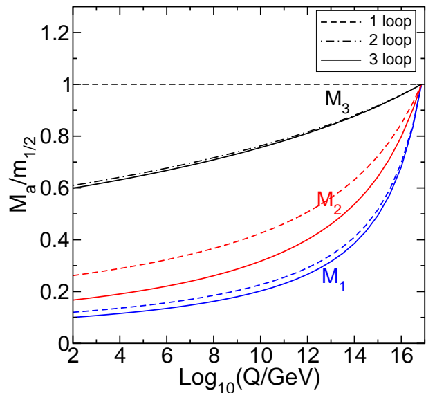
FIG. 4: Running of gaugino masses in the QUE model, assuming a unified value m_{1/2} at M_{\text{unif}} . The gluino mass parameter M_3 is evolved according to the 1, 2, and 3 loop beta functions in the top three lines. The 1 and 3 loop beta functions are shown for the parameters M_1 (bottom two lines) and M_2 , for which the 2-loop and 3-loop results are not visually distinguishable. Note the significant running of M_3 due to multi-loop effects.
