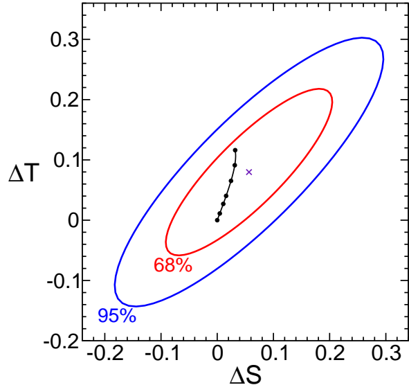
FIG. 9: Corrections to electroweak precision observables S, T from the LND model at the fixed point (k_N, h_N) = (0.765, 0) , for varying M_L = M_N = m_{\tau'} > 100 GeV, in the limit of heavy scalar superpartners. The seven dots on the line segment correspond to m_{\tau'} = 100, 120, 150, 200, 250, 400 GeV and \infty , from top to bottom. The experimental best fit is shown as the \times at (\Delta S, \Delta T) = (0.057, 0.080) . Also shown are the 68% and 95% CL ellipses, obtained as described in the text. The point \Delta S = \Delta T = 0 is defined to be the Standard Model prediction for m_t = 173.1 GeV and m_{h^0} = 115 GeV.
