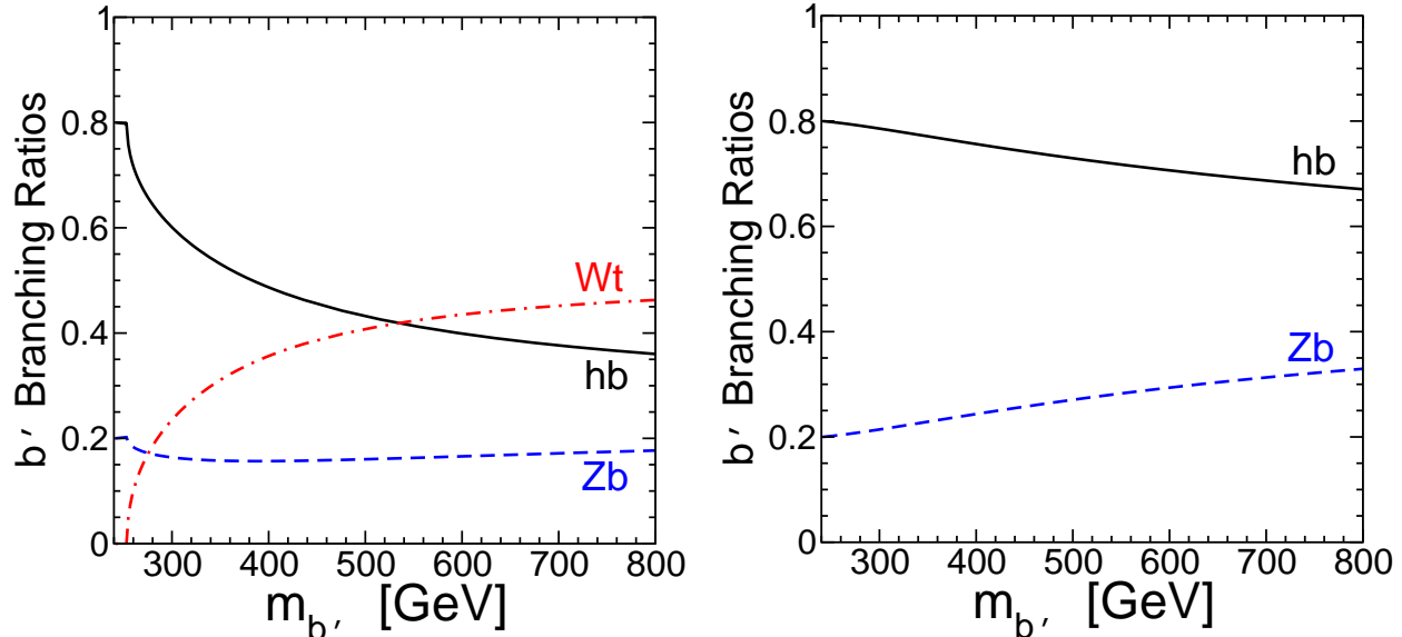
FIG. 15: Branching ratios for the lightest extra quark, b'_1 , in the QDEE model with M_Q = M_D , to final states Wt , Zb , and h^0b . The left panel shows the “democratic” case that \epsilon_D dominates, and the right panel shows the “ W -phobic” case that \epsilon'_D dominates, leading to mostly neutral-current decays. In the “ W -philic” case that \epsilon_U dominates leading to mostly charged-current decays, then BR(b'_1 \rightarrow Wt) = 1 (not shown).
