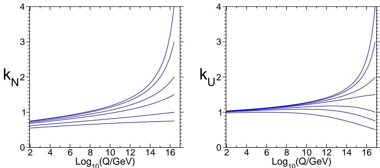
FIG. 2: Renormalization group trajectories near the fixed point for k_N in the LND model (left panel) and k_U in the QUE model (right panel), showing the infrared-stable quasi-fixed point behaviors. Here m_t = 173.1 GeV and \tan\beta = 10 are assumed.
