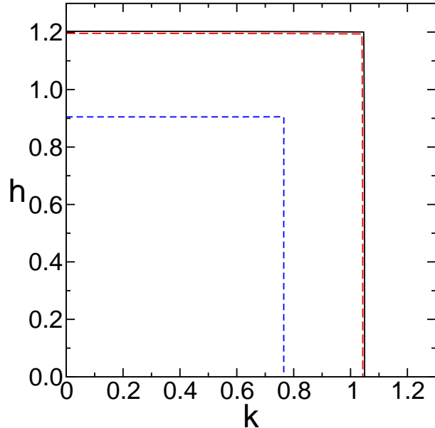
FIG. 3: The contours represent the infrared-stable quasi-fixed points of the 2-loop renormalization group equations in the plane of Yukawa couplings (k_i, h_i) evaluated at Q = 500 GeV. The allowed perturbative regions (defined by k_i, h_i < 3 at Q = M_{\text{unif}} ) are to the left and below the contours. The long dashed (blue) line corresponds to k_N, h_N in the LND model. The solid (black) line corresponds to k_U, h_U in the QUE model, and the nearly overlapping short dashed (red) line corresponds to k_D, h_D in the QDEE model. Here m_t = 173.1 GeV and \tan \beta = 10 are assumed. The very nearly rectangular shape of these contours reflects the absence of direct coupling between the Yukawa couplings in the one-loop \beta functions.
