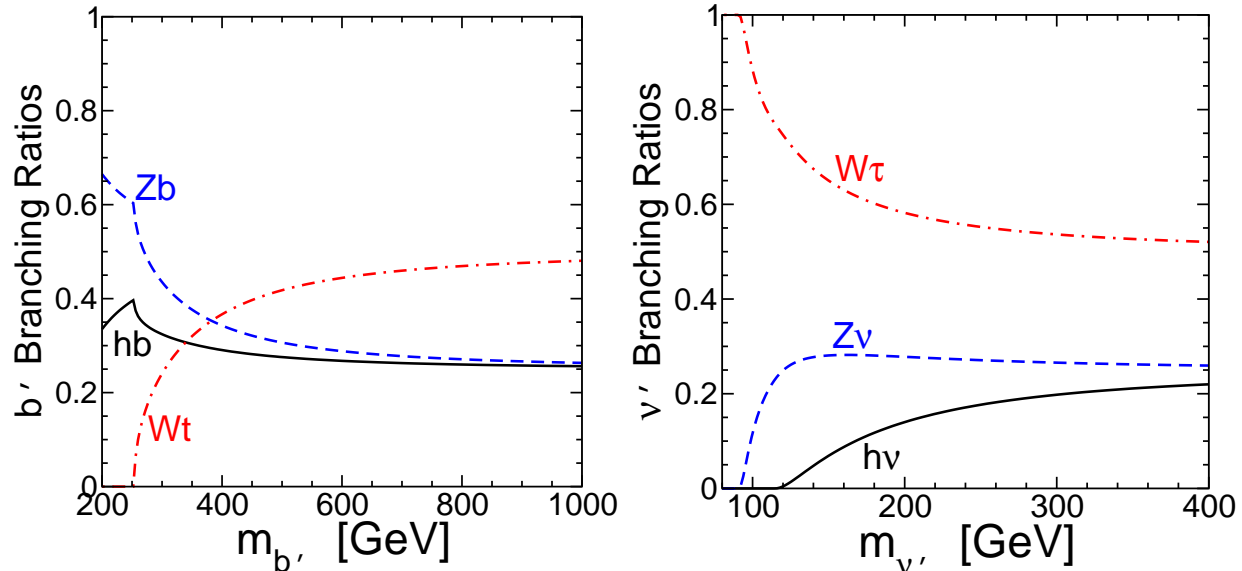
FIG. 12: The branching ratios of the lightest new quark b' (left panel) and the lightest new lepton \nu'_1 (right panel) in the LND model. The \nu'_1 results assume that \epsilon_N \gg \epsilon_E ; if instead \epsilon_E \gg \epsilon_N then BR(\nu'_1 \rightarrow W\tau) = 1 (not shown).
