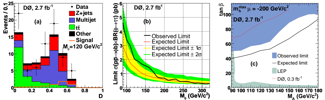
FIG. 1: (a) The distribution of the final discriminant variable, D = NN_{top} \times LL_{MJ} . The figure includes all \tau Types. (b) The cross-section limit as a function of Higgs boson mass. (c) The region in the \tan\beta versus M_A plane excluded by this analysis, LEP neutral MSSM Higgs searches, and the previous D0 result in this channel.
