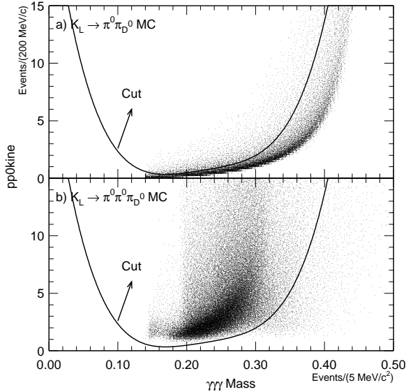
FIG. 4: The pp0kine variable plotted versus the \gamma\gamma\gamma invariant mass for a) K_L \rightarrow \pi^0 \pi_D^0 and b) K_L \rightarrow \pi^0 \pi^0 \pi_D^0 Monte Carlo events. The dark line represents the cut indicated in the text.
