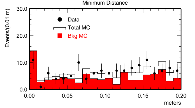
FIG. 5: The minimum distance between the projection of the upstream electron track segment to the CsI calorimeter and any photon candidate. The dots represent the data and the solid histogram the sum of the background and signal Monte Carlo. The enhancement at low values of the minimum distance is the result of bremsstrahlung production.
