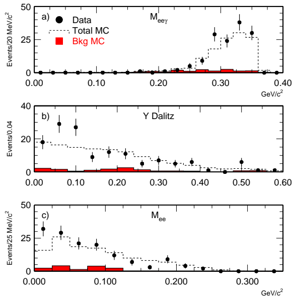
FIG. 7: The Dalitz variables used in the fit for a_V : a) m_{e^+e^-\gamma} , b) Y and c) m_{e^+e^-} . The dots are the data. The dashed histogram is the sum of the background and signal Monte Carlo, and the filled histogram is the background Monte Carlo.
