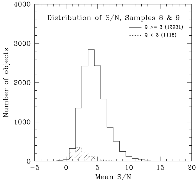
Figure 7. Histograms of mean S/N per pixel for all Sample 8 and 9 spectra which gave reliable redshifts (solid line) and for those which failed (dotted line, shaded histogram). 95% of spectra with S/N > 2 are adequate for determining redshifts.
