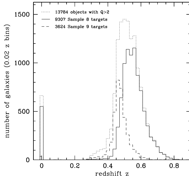
Figure 9. Redshift histograms for the 2SLAQ LRGs. The solid line is for those objects in the primary sample (8) and the dashed line is for the secondary sample (9). The histogram for all objects with reliable redshifts is shown as a dotted line. The spike at z = 0 represents the 5% contamination by foreground M-stars. The effectiveness of the 2SLAQ photometric selection for z \sim 0.5 galaxies is evident.
