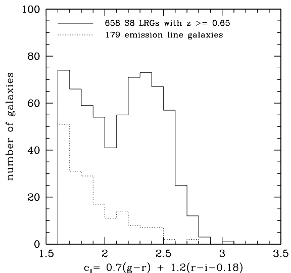
Figure 13. A histogram of the distribution of the c_{\parallel} photometric parameter for galaxies in the primary LRG sample with z \geq 0.65 and \sigma_g < 0.35 . The full line is for all LRGs, the dotted line is for those with [O II] emission. The sharp boundary at c_{\parallel} = 1.6 marks the LRG colour selection cut-off. The bins are independent, supporting the reality of the dip in the full distribution at c_{\parallel} = 2 . The highly skewed distribution of emission line galaxies indicates the existence of two separate populations of high redshift galaxies, with only the redder peak corresponding to true LRGs.
