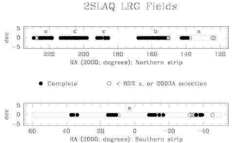
Figure 2. Layout of the 2dF 2SLAQ fields within the northern (upper) and southern (lower) Galactic strips. Filled circles denote fully observed fields, i.e. with redshift completeness \geq 85\% . Open circles represent fields with completeness < 85\% or with non-standard selection criteria. The letters ‘a’-‘e’ and ‘s’ signify the sub-strips and are used as the first character of the field names.
