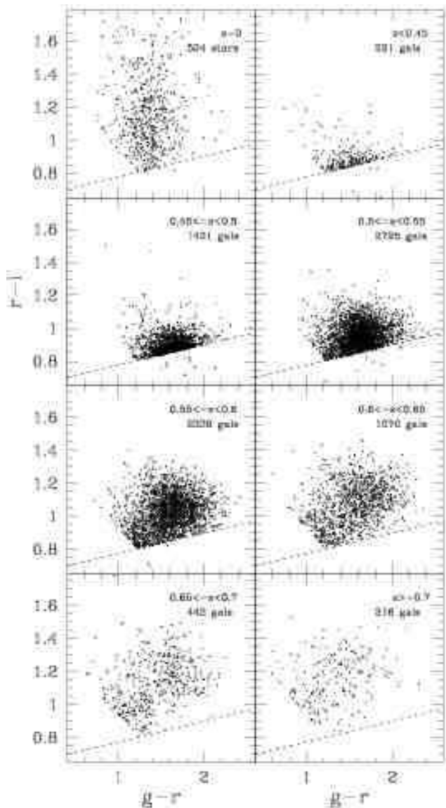
Figure 12. The distribution of LRGs in the 2-colour ( r-i ) versus ( g-r ) diagram as a function of z , for the primary (Sample 8) objects. Each panel is for a successively larger redshift range, starting with the M-type stars at top left and ending with the highest redshift objects at bottom right. The dotted line in each panel is the d_{\perp} = 0.65 lower boundary to Sample 8, for reference (a few points appear below this line due to revisions of the photometry). The main clump of LRGs moves to redder r-i colours at approximately constant g-r as z increases, as the 4000\text{\AA} break moves through the r -band.
