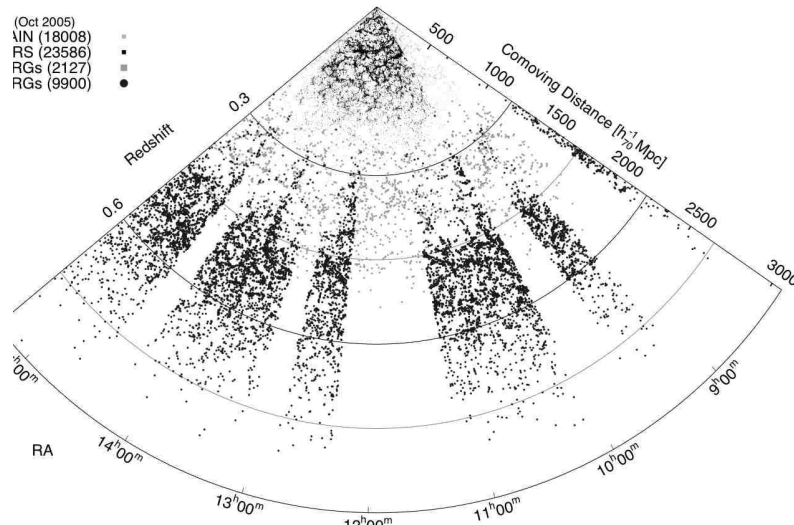
Figure 15. A wedge diagram plotting redshift or distance as a function of RA for all the 2SLAQ LRGs in the Northern Galactic strip (large black points in discrete sectors). Very small points with z < 0.3 show the 2dFGRS and SDSS MAIN galaxies of all types and the grey points at intermediate redshifts are from the SDSS LRG survey, all lying within the same 2^\circ -wide strip. Considerable structure is evident within the LRG samples, similar to what is seen at much lower redshifts.
