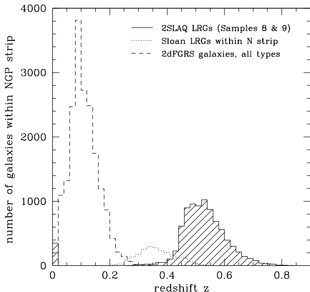
Figure 10. The redshift distribution of three surveys in the same 2^\circ -wide Northern equatorial strip. The 2SLAQ LRG redshift distribution (shaded histogram) is compared with that of the SDSS LRG survey (dotted line) and galaxies of all types in the 2dFGRS (dashed line).
