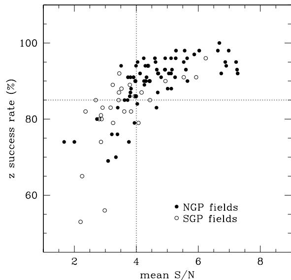
Figure 4. The redshift success rate for each dataset as a function of mean S/N per pixel per object. The redshift completeness can fall catastrophically when the mean S/N is below 4.0 (vertical dotted line): the observations were repeated for most such datasets. The horizontal dotted line marks the 85% success rate used as the threshold for deciding that the observations of a field were complete.
