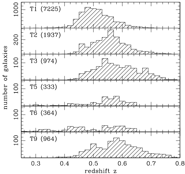
Figure B2. Histograms of the redshifts for which each of the templates was used, for Sample 8 and 9 galaxies, omitting the little-used A- and K-type spectra and the M-type spectrum which fitted only foreground M-stars. The numbers of galaxies in each panel are given in parentheses: note the different ordinate scales in the top two panels.
