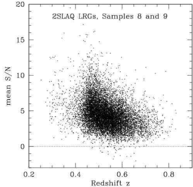
Figure 8. Mean S/N as a function of redshift z , for all primary (Sample 8) and secondary galaxies with reliable redshifts. A few objects fall below the S/N = 0 boundary (dotted line) due to errors in sky subtraction, but retain sufficient features for a reliable redshift determination.
