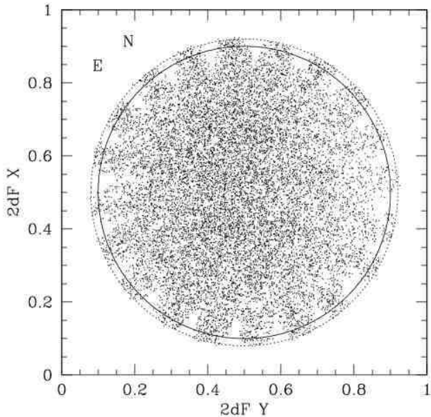
Figure 3. The distribution of LRG targets across the 2dF field, with north to the top and east to the left. The dotted circle represents the nominal 2.1^\circ field diameter; the solid circle at 1^\circ radius indicates the effective area covered. The empty triangles around the edge are inaccessible to the fibres feeding the single spectrograph used for the LRGs. The lower density towards the right-hand side of the field is due to the allocation of 20–30 of the western fibres to sky: those fibres feed the central rows in the spectrograph camera.
