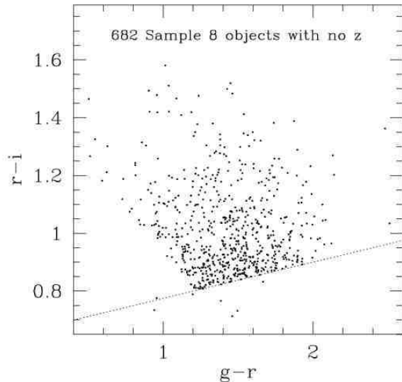
Figure 14. The 2-colour distribution of the 8% of primary (Sample 8) LRGs with unreliable redshifts, i.e. with redshift quality Q < 3 (again omitting data with \sigma_g > 0.35 ). This distribution is significantly different from that of the full sample or any of the redshift sub-samples plotted in Fig. 12. A relatively high proportion of objects with extreme colours fail to give good redshifts, while bona fide LRGs in the clump with z \sim 0.55 are under-represented. The ‘failed redshift’ objects include a mixture of high redshift galaxies, galaxies with peculiar spectra, composite objects, lower redshift galaxies which are not LRGs, and LRGs which simply had weak spectra because of bad fibre placement or low throughput.
