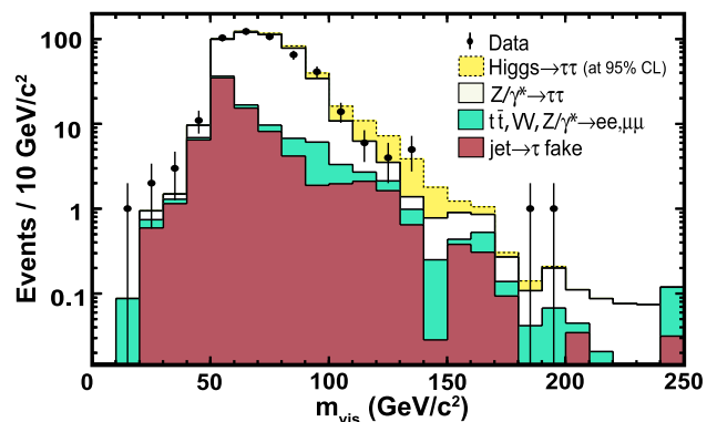
FIG. 2: Example fit of the m_{vis} distribution for signal with m_A = 140 GeV/ c^2 . Signal and background normalizations correspond to the fit results for signal exclusion at 95% CL.
