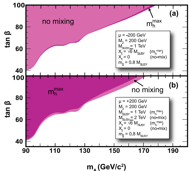
FIG. 4: Excluded regions in the \tan\beta vs m_A plane for the m_h^{max} and no-mixing scenarios with (a) \mu < 0 and (b) \mu > 0 .
