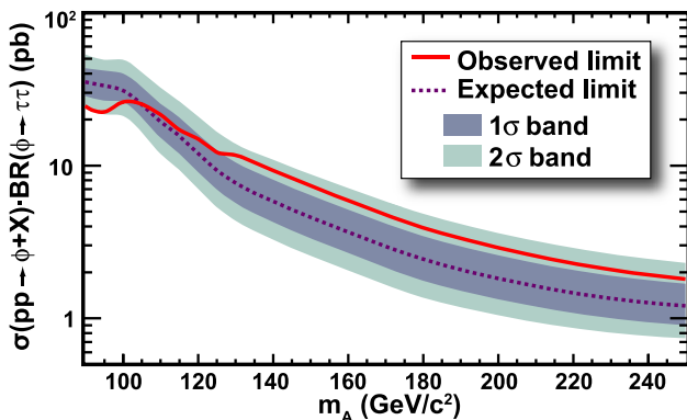
FIG. 3: Upper limits at 95% CL on Higgs production cross section times branching fraction to \tau pairs. The expected limits from the pseudo-experiments are also shown.
