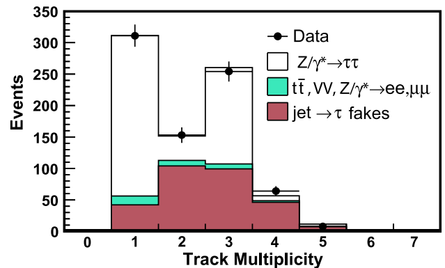
FIG. 1: Track multiplicity for hadronically decaying tau candidates before applying the opposite charge and N_{trk}^{sig} requirements.
