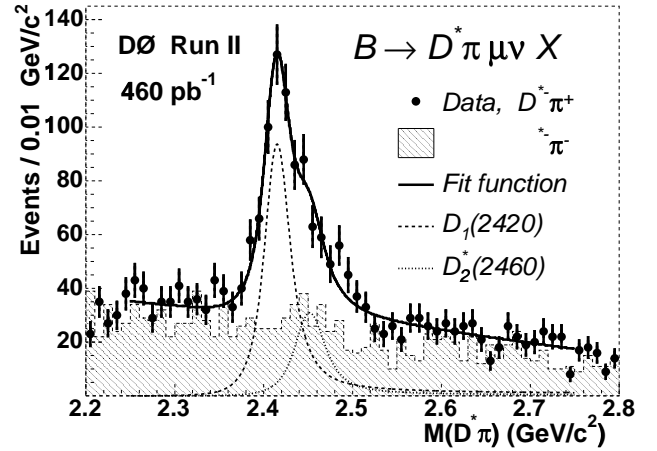
FIG. 2: The invariant mass M(D^*\pi) . Event selection is described in the text. The points correspond to the D^*\pi combinations with opposite charges, and the hatched histogram corresponds to the same-charge combinations. The distribution was fit with a sum of two relativistic Breit-Wigner functions corresponding to two narrow D^{**} states and a second-order polynomial describing the background. The contributions of D_1^0 and D_2^0 to the fit are shown separately.
