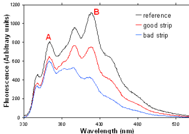
Fig. 9. Fluorescence spectra of three extruded scintillator samples: in black, the reference; in red, from a strip with good response; and in blue, from a strip with lower response.
