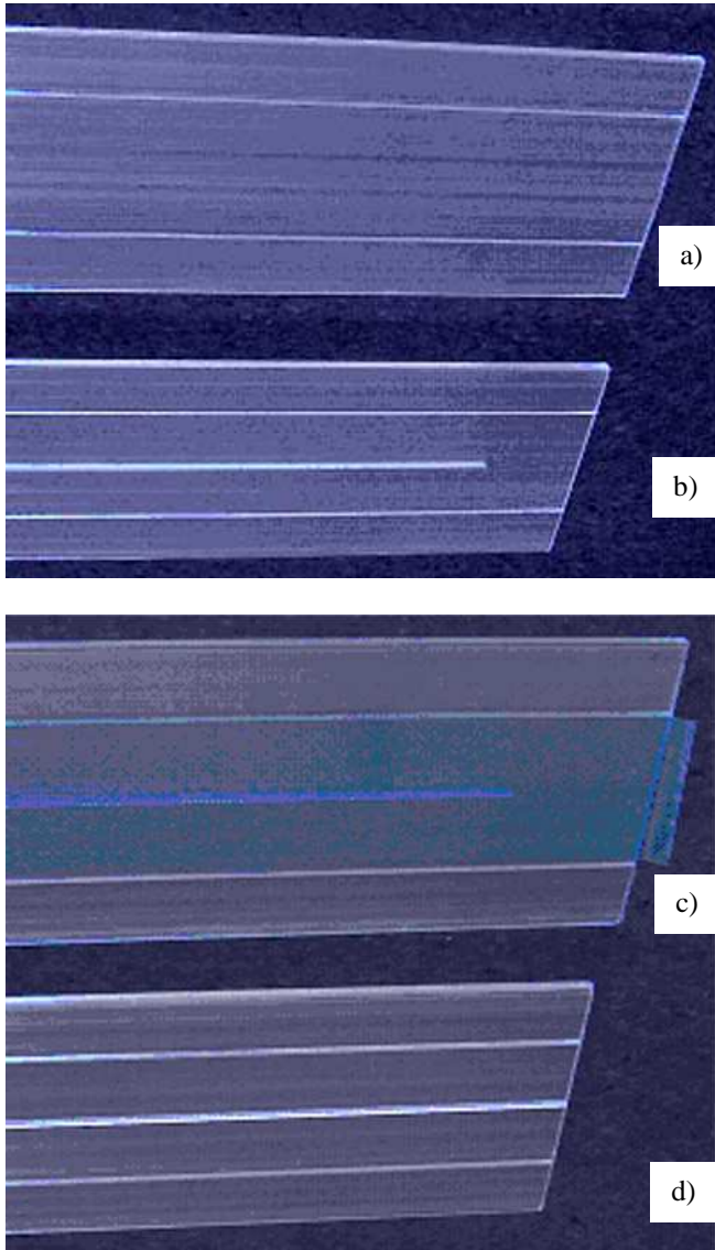
Fig. 1. a) a strip after extrusion; b) the same strip with a machined separation groove; c) the strip with blue tape; d) the trimmed strip with the glued separation groove.
