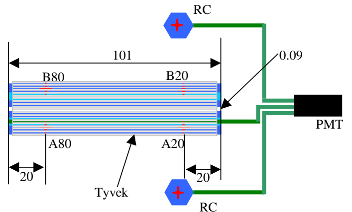
Fig. 2. Schematic of the setup used for strip measurements. (All dimensions are given in cm). The letters RC denote the reference cells.
