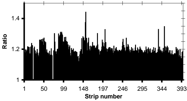
Fig. 7. Ratio A20/A80 versus number of the strips.
