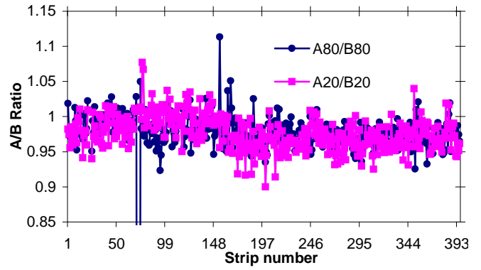
Fig. 8. Asymmetry across the strip (the strip number is not associated with production time).
