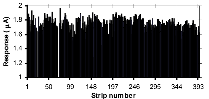
Fig. 5. Strip responses as measured at position A20.
