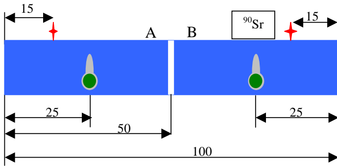
Fig. 3. A schematic used for a strip orientation and a radioactive source positioning. (all dimensions are given in mm).
