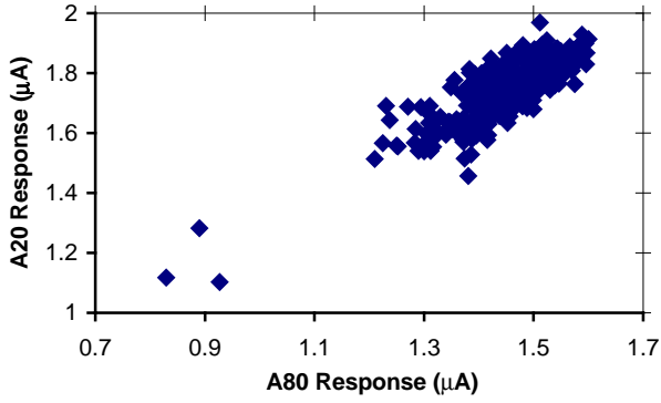
Fig. 6. A20 response versus A80 (for all strips) illustrates the brightness (at 20) and attenuation (at 80) for each strip.
