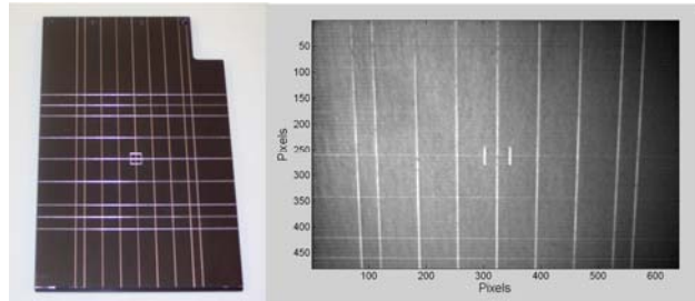
Figure 4: Left image shows photograph of target used to measure OTR detector optical distortion. Right image is of distortion target taken with OTR detector.
