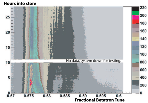
Figure 3: Water-fall tune spectra taken during a typical store.
