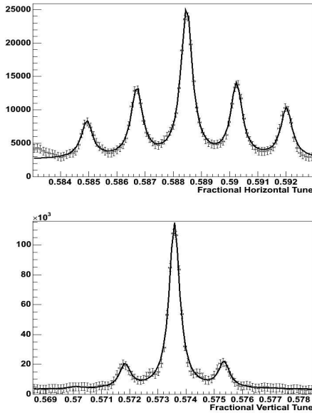
Figure 1: Horizontal (top) and Vertical (bottom) tune spectra of uncoalesced beams on the central orbit
