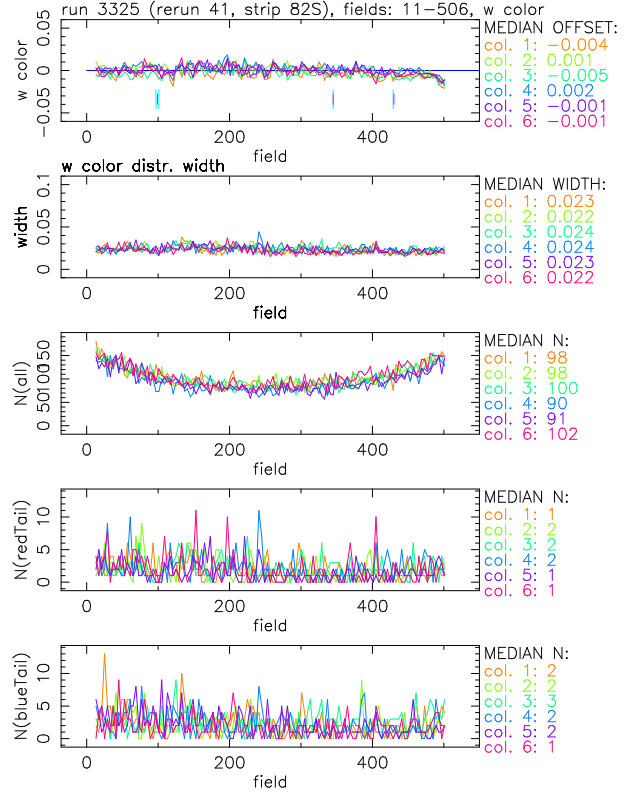
N(\text{All}) is the number of all w stars N(\text{redTail}) is the number of stars with w > 2 \cdot \sigma(w) N(\text{blueTail}) is the number of stars with w < 2 \cdot \sigma(w) The data are binned every 4 fields (cyan/magenta: BAD/HOLE field)
