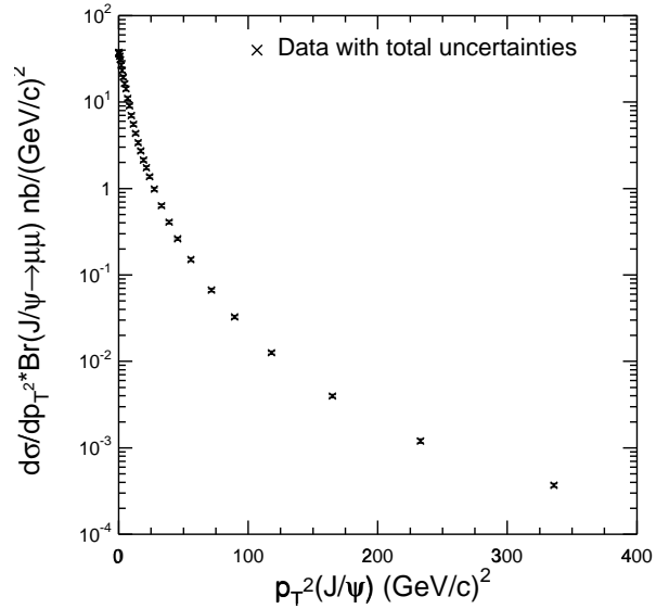
FIG. 9: The invariant J/\psi cross section, d\sigma/dp_T^2 \cdot Br(J/\psi \rightarrow \mu\mu) , as a function of p_T^2(J/\psi) . The differential cross section is plotted. This includes correlated uncertainties.
