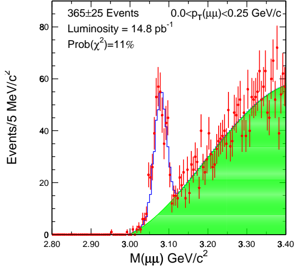
FIG. 2: Invariant mass distribution of reconstructed J/\psi \rightarrow \mu\mu events in the range p_T(\mu\mu) < 0.25 GeV/ c . The points with error bars are data. The solid line is the fit to the signal shape from the simulation and a third order polynomial for the background. The shaded histogram is the fitted background shape. The number of signal events and the fit probability of the binned \chi^2 fitting are also provided.
