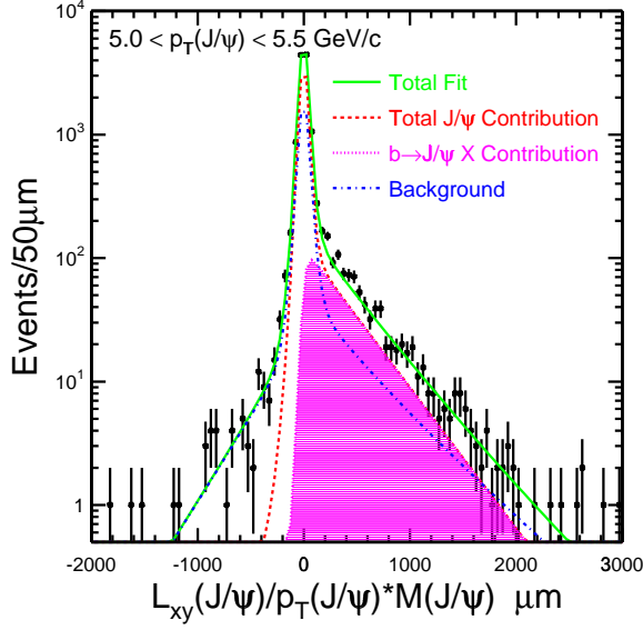
FIG. 11: Fits to the J/\psi pseudo-proper decay time in the range 5.0 < p_T(\mu\mu) < 5.5 \text{ GeV}/c to extract the fraction of events from long-lived b -hadron decays. The solid line is the fit to all the events in the mass window, the dashed line is the fit to all signal events, the solid histogram is the fit to the portion of the signal events that are from b -hadron decays and the dot-dashed line is the fit to background events.
