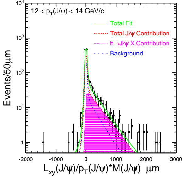
FIG. 12: Fits to the J/\psi pseudo-proper decay time in the range 12.0 < p_T(\mu\mu) < 14.0 GeV/c to extract the fraction of events from long-lived b -hadron decays. The solid line is the fit to all the events in the mass window, the dashed line is the fit to all signal events, the solid histogram is the fit to the portion of the signal events that are from b -hadron decays and the dot-dashed line is the fit to background events.
