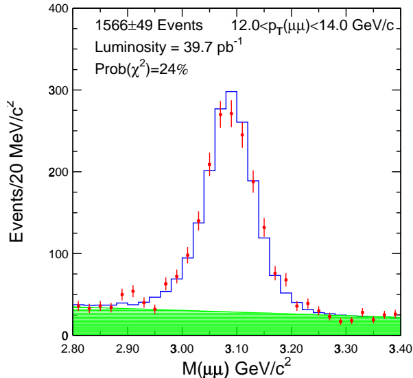
FIG. 5: Invariant mass distribution of reconstructed J/\psi \rightarrow \mu\mu events in the range 12.0 < p_T(\mu\mu) < 14.0 GeV/c. The points with error bars are data. The solid line is the fit to the signal shape from the simulation and a linear background. The shaded histogram is the fitted background shape.
