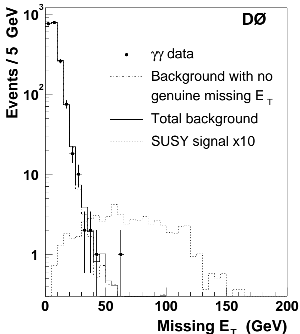
FIG. 1: The \cancel{E}_T distribution for the diphoton and background samples. Also shown is the expected distribution for the GMSB point with \Lambda = 80 TeV, multiplied by a factor of ten.
