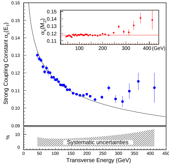
FIG. 1: The strong coupling constant as a function of E_T for \mu_R = E_T measured using CTEQ4M parton distributions. The shaded area shows the experimental systematic uncertainties. The curved line represents the NLO QCD prediction for the evolution of \alpha_s(E_T) using \alpha_s(M_Z) = 0.1178 , the average value obtained in the region 40 < E_T < 250 GeV. The \alpha_s(M_Z) extracted from \alpha_s(E_T) is shown in the inset along with the weighted average as the horizontal line.
