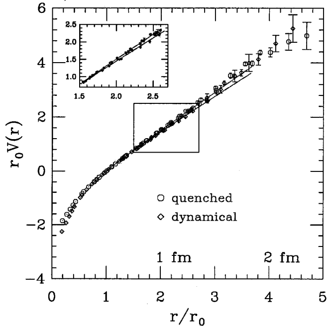
Figure 1. The ground state static quark potential for quenched (octagons) and 2+1 flavor (diamonds) QCD, in units of r_0 . The solid lines are fits to the Coulomb plus constant plus linear form, fixing V_{\text{fit}}(r_0) = 0 . The lattice spacing is matched using r_0 . The inset expands the area shown by the box.
