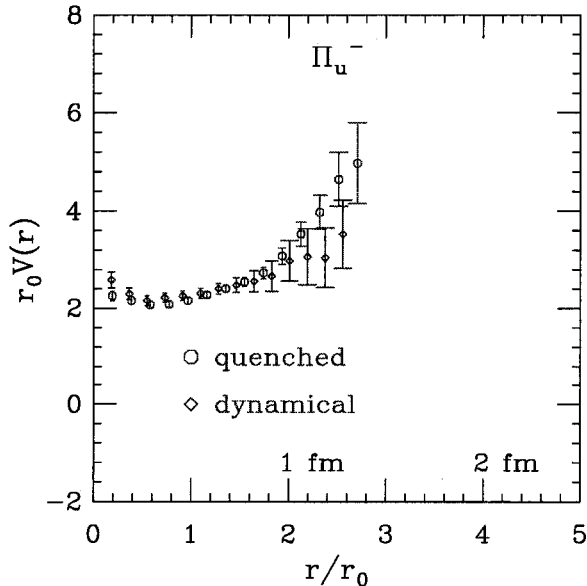
Figure 3. The \Pi_u^- potential for quenched (octagons) and 2+1 flavor (diamonds) QCD, in units of r_0 . The potentials are plotted relative to the zero determined in the fit to the ground state potentials.
