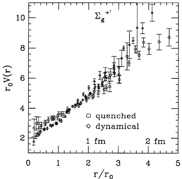
Figure 2. The excited \Sigma_g^{+'} potential for quenched (octagons) and 2+1 flavor (diamonds) QCD, in units of r_0 . The lattice spacing was matched using r_0 .
