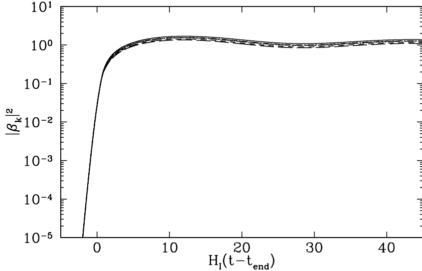
FIG. 2: The absolute square of the Bogoliubov coefficient as a function of time for several different values of B and C ( B is dimensionless and C is in units of M_{\text{Pl}}^2 .) We have g = 0.01 , \lambda = 1 , M_X = 0.1H_0 , and k = 0.1a_iH_0 . The lines correspond to the deformation parameters (B, C) given by (1, 10^9) ; (10^3, 10^7) ; (10^5, 10^3) ; (10^5, 10^5) ; (10^5, 10^7) ; (10^5, 10^9) . The lines are hard to distinguish on this scale and asymptotically approach within 10% of each other.
