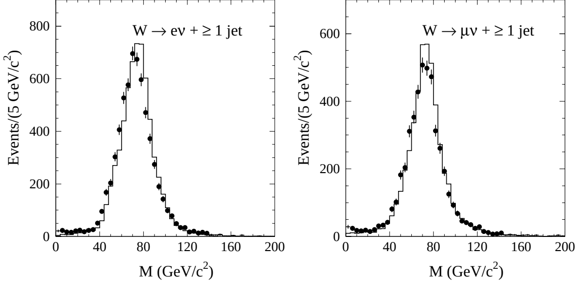
FIG. 2. Distribution of the transverse mass M of W candidates in the data ( \bullet ) and in a simulation using the Herwig generator (solid histogram). We utilize measured quantities without the full set of corrections used to determine the W mass.
