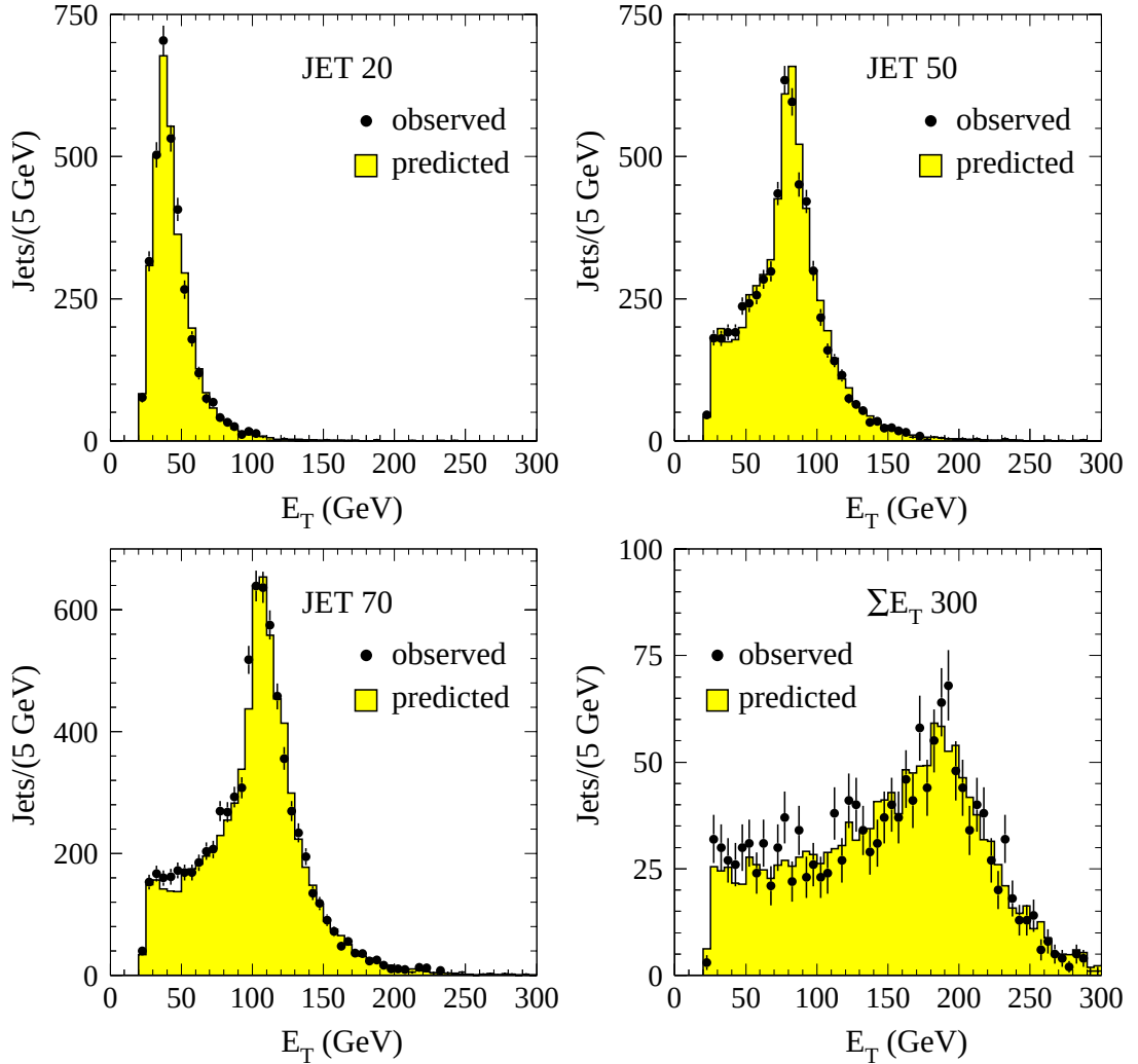
FIG. 27. Transverse energy distributions of jets with a negative JPB tag. The 4 samples were used for the construction of the mistag probability matrix.
