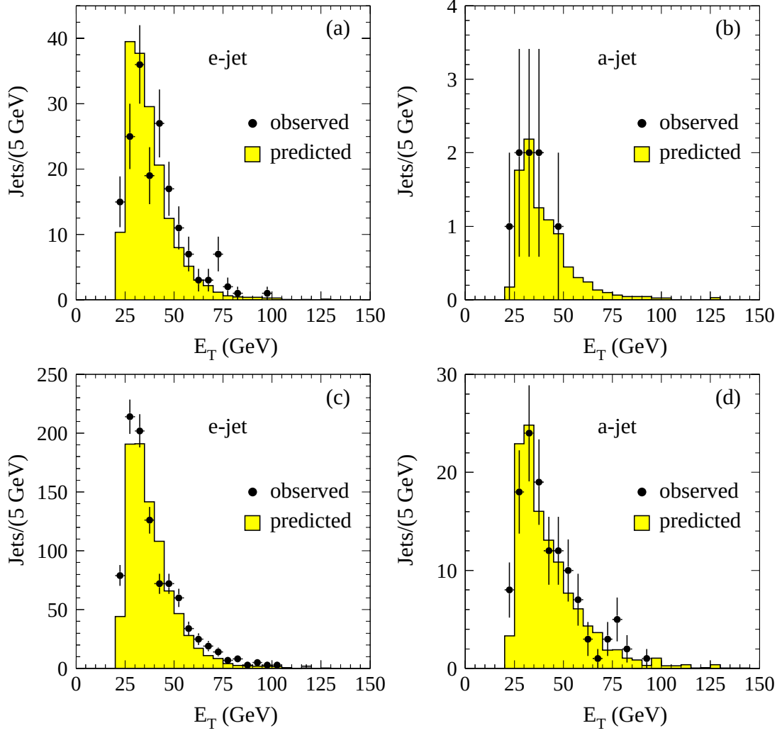
FIG. 26. Transverse energy distributions in the inclusive electron simulation. In (a) e-jets with negative SECVTX tags; (b) a-jets with negative SECVTX tag; (c) e-jets with negative JPB tags; (d) a-jets with negative JPB tag.
