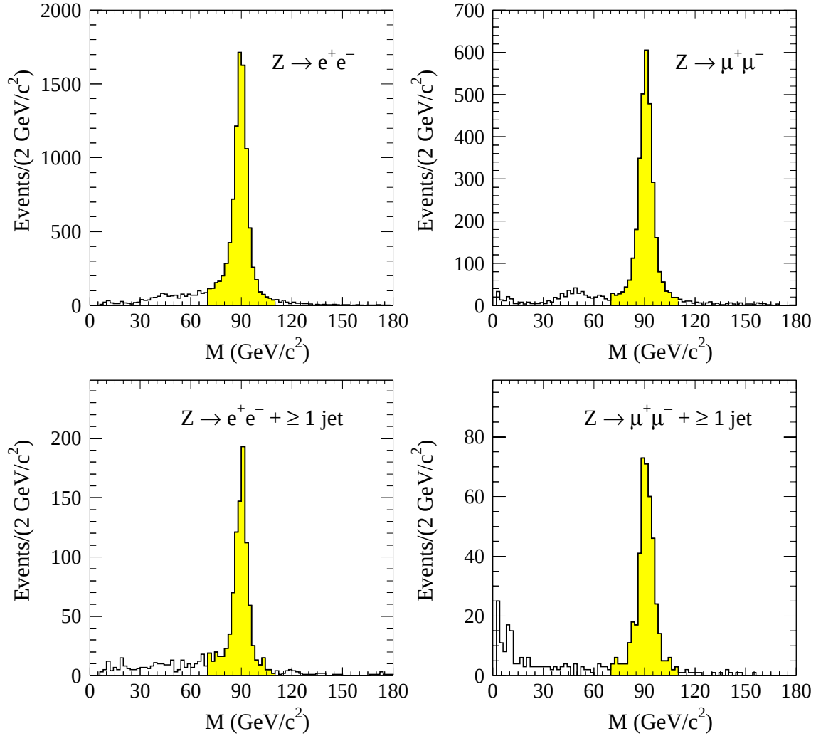
FIG. 1. Invariant mass distributions of electron and muon pairs before and after requiring the presence of at least one jet with E_T \geq 15 GeV and |\eta| \leq 2 . The shaded area indicates the mass window used to select Z candidate events.
