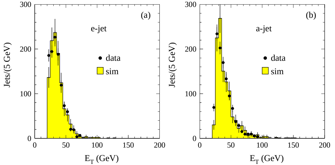
FIG. 11. Distributions of the transverse energy of electron-jets (a) and away-jets (b) in events with double SECVTX tags.
