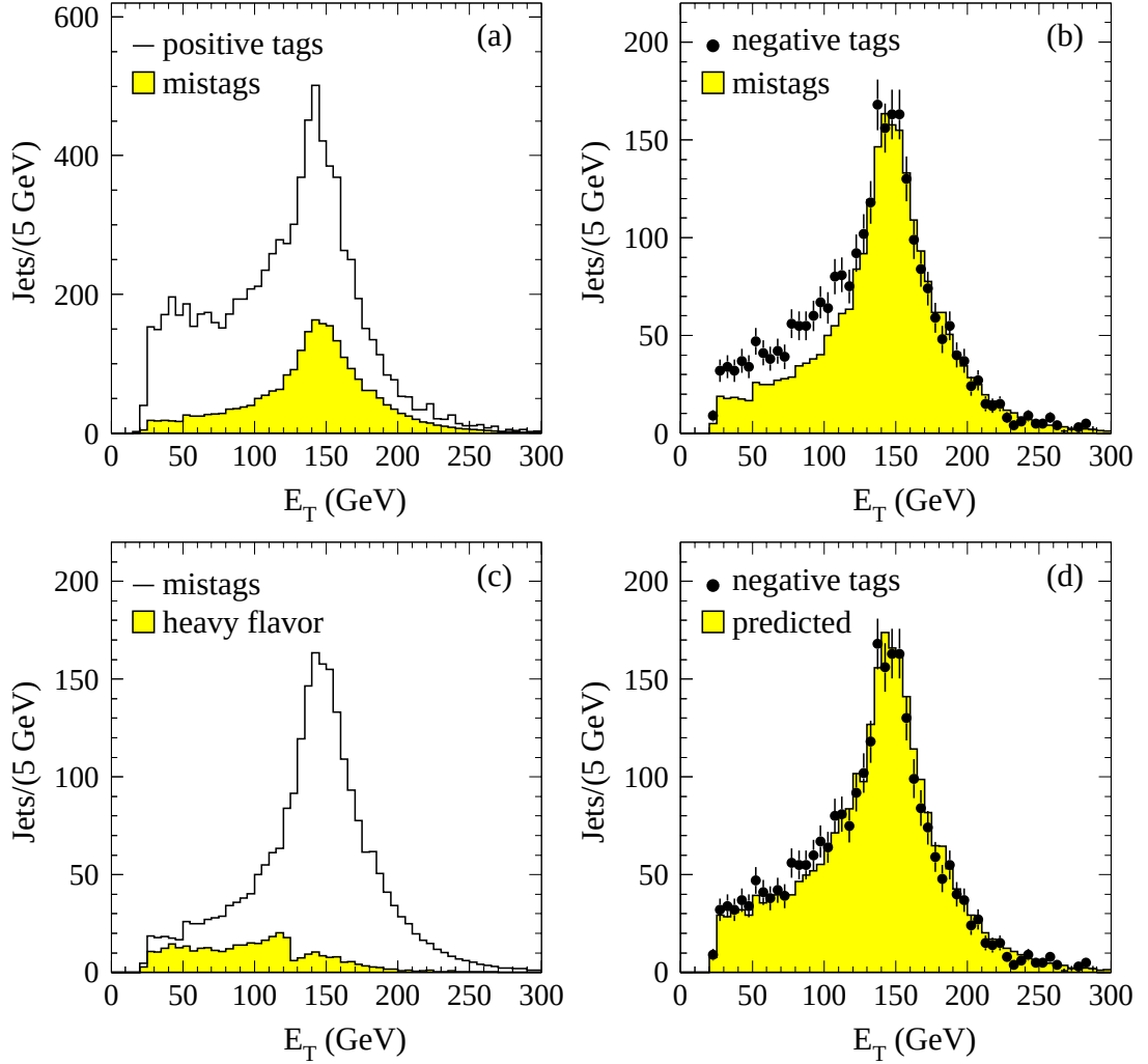
FIG. 21. E_T distributions of jets with SECVTX tags in the JET 100 sample. On (a), observed positive tags (histogram) are compared to the predicted mistags (shaded histograms). On (b), observed negative tags ( \bullet ) are compared to the predicted mistags (shaded histograms). On (c), predicted mistags (histogram) are compared to the predicted heavy flavor contribution to the negative tags (shaded histograms). On (d), observed negative tags ( \bullet ) are compared to the sum of the predicted mistags and heavy flavor contribution to the negative tags (shaded histogram).
