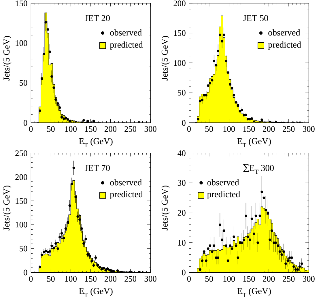
FIG. 22. Transverse energy distributions of jets with negative SECVTX tags. The 4 data samples were used for the construction of the mistag probability matrix.
