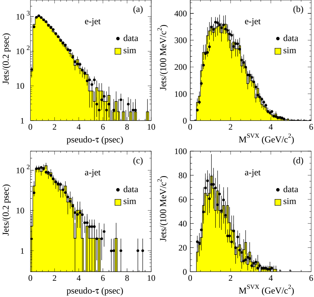
FIG. 12. Distributions of pseudo- \tau (a) and of the invariant mass (b) of SECVTX tags in electron-jets; (c) and (d) are the analogous distributions for away-jets in events with double tags.
