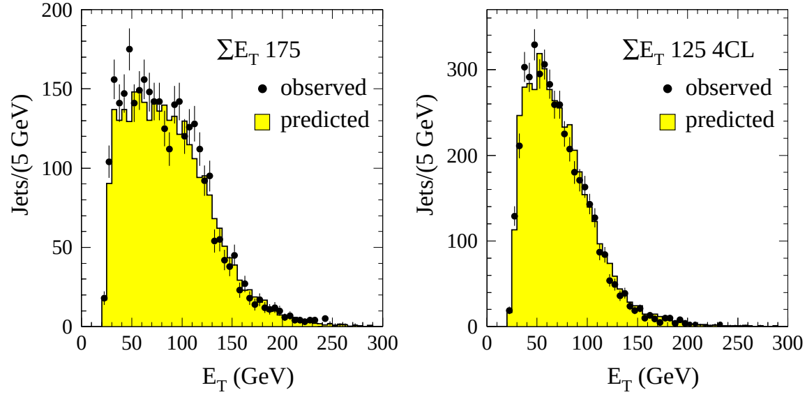
FIG. 28. Transverse energy distributions of jets with negative JPB tags in the \Sigma E_T 175 (a) and \Sigma E_T 125 4CL (b) samples, which were not used for the construction of the mistag probability matrix.
