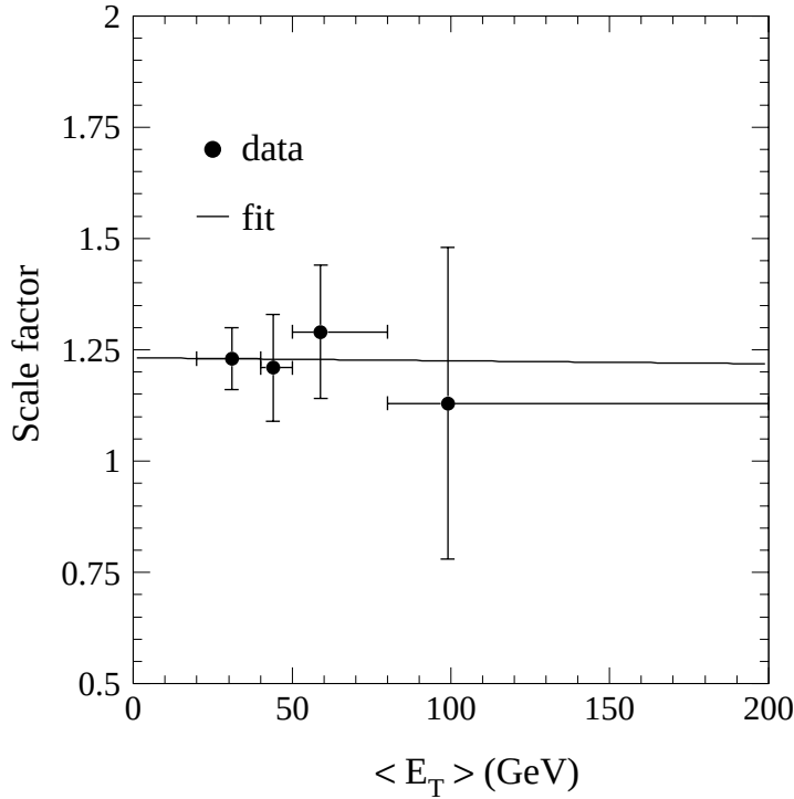
FIG. 13. SECVTX tagging efficiency scale factor as a function of the average transverse energy \langle E_T \rangle of the electron-jet. The line represents a fit with a first degree polynomial.
