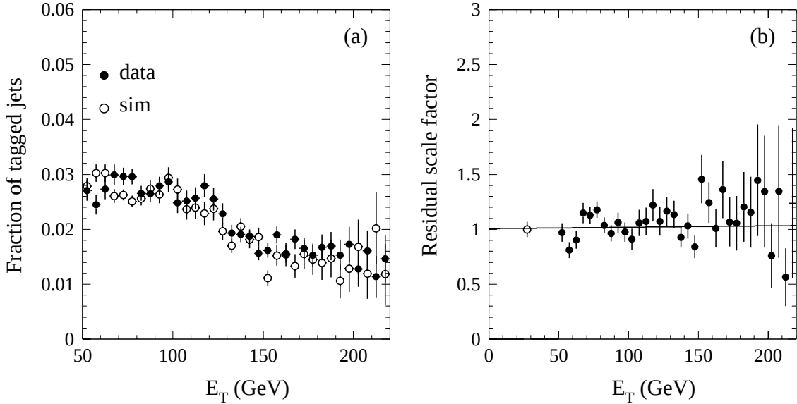
FIG. 14. Fractions of tagged jets (a) as a function of the jet transverse energy. The residual scale factor (b) is defined as the ratio of these fractions in the data and the simulation. The open circle in (b) represents the inclusive electron sample result.
