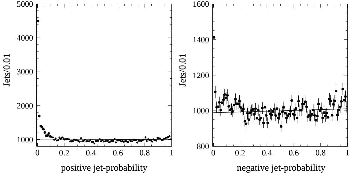
FIG. 5. Distributions of positive and negative jet-probability in a mixture of JET 50 and JET 140 data. The lines represent a fit to the negative distribution with a first order polynomial. The slope of the fit corresponds to a 1.6% change of the distribution over the entire jet-probability range.
