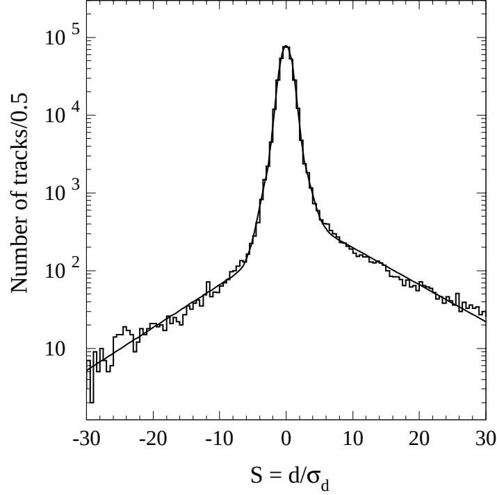
FIG. 3. Distribution of the signed impact parameter significance of tracks in the JET 50 sample. The resolution function \mathcal{R}(S) is the result of a fit using two Gaussians plus an exponential function, separately for the positive and negative sides.
