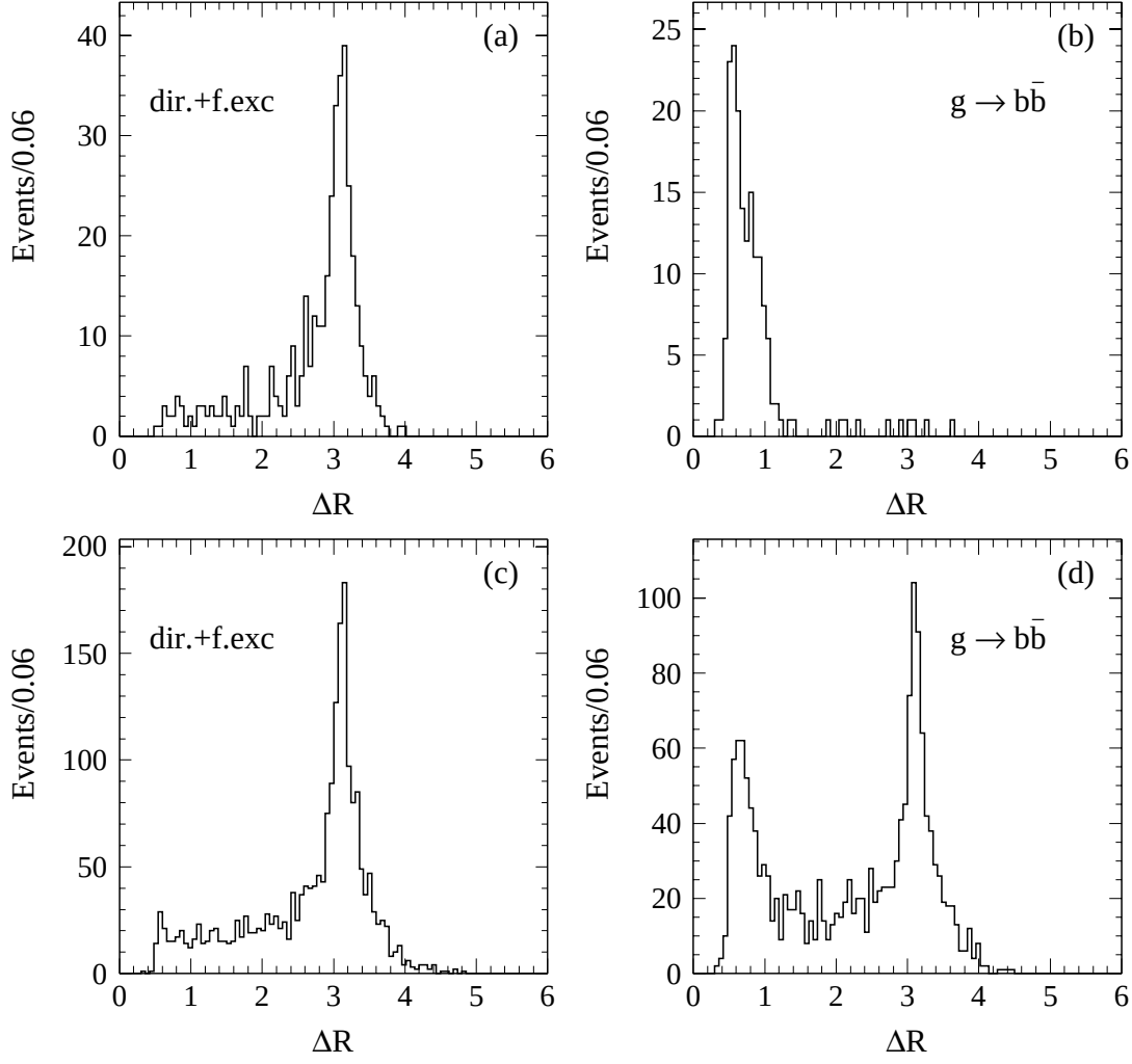
FIG. 30. Distributions of the distance \Delta R between two b -jets tagged by SECVTX in JET 50 simulated events contributed by (a) direct production and flavor excitation or (b) gluon splitting. (c) and (d) are the distributions of the distance between a b -jet tagged by SECVTX and the closest jet in the event with E_T \geq 10 GeV.
