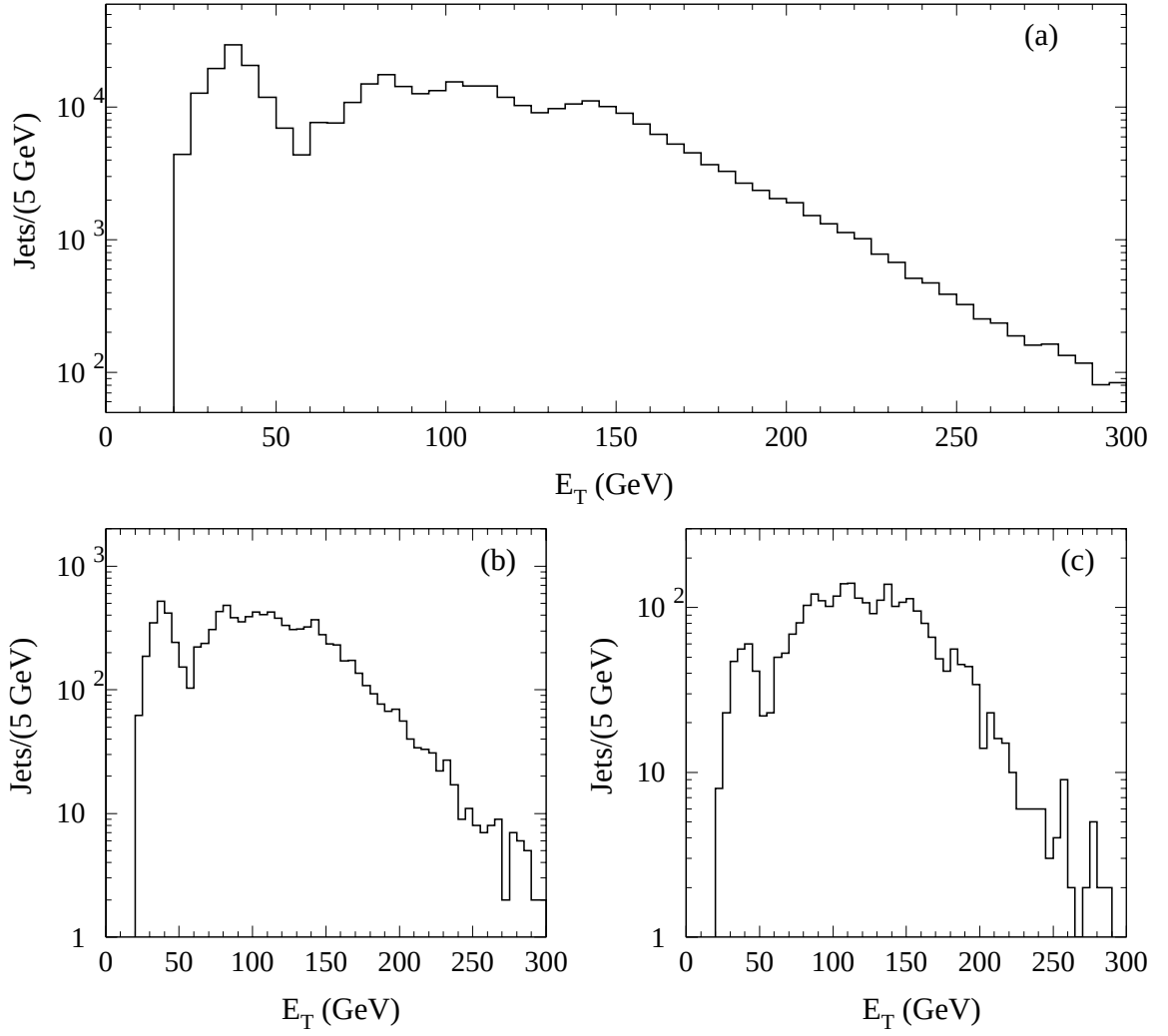
FIG. 15. Transverse energy distributions of (a) taggable jets , and jets with positive (b) and (c) negative SECVTX tags.
