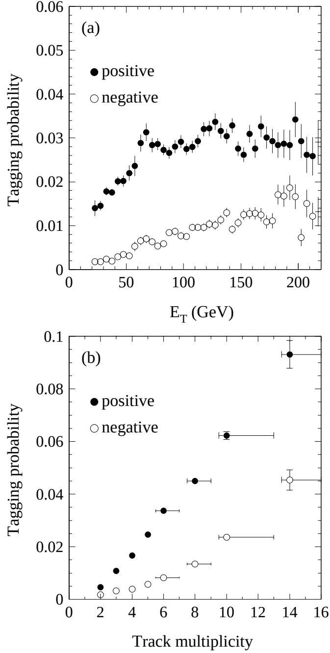
FIG. 17. The positive and negative SECVTX tagging probability as a function of (a) the jet E_T and (b) the number of SVX tracks in a jet.
