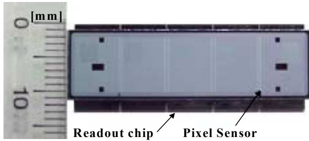
Figure 13: 5-chip Pixel Module with Indium Bumps
