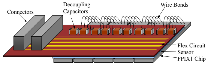
Figure 5: Sketch of the Pixel Multichip Module
