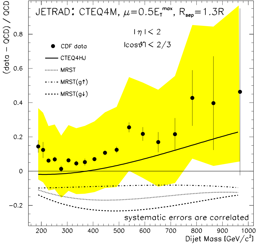
Figure 1: The fractional difference between the measured differential cross section and the QCD prediction (points) as a function of dijet mass. The band is the systematic uncertainty. The curves are the fractional difference between other QCD predictions, for various choices of parton distributions, and our default QCD prediction using CTEQ4M.
