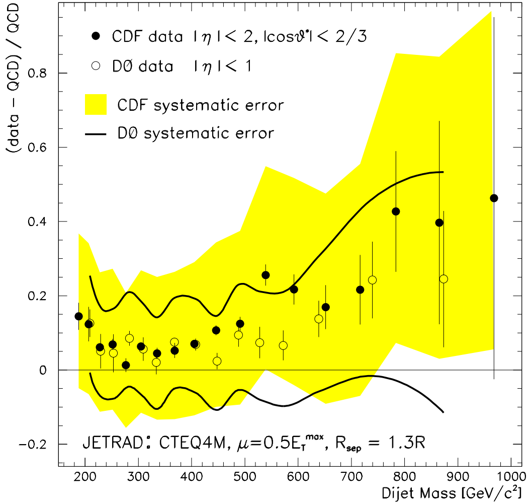
Figure 2: The difference between CDF data and QCD (solid points as shown in Fig. 1) compared to the difference between DØ data [4] and QCD (open points). The solid curves are the DØ systematic uncertainty.
