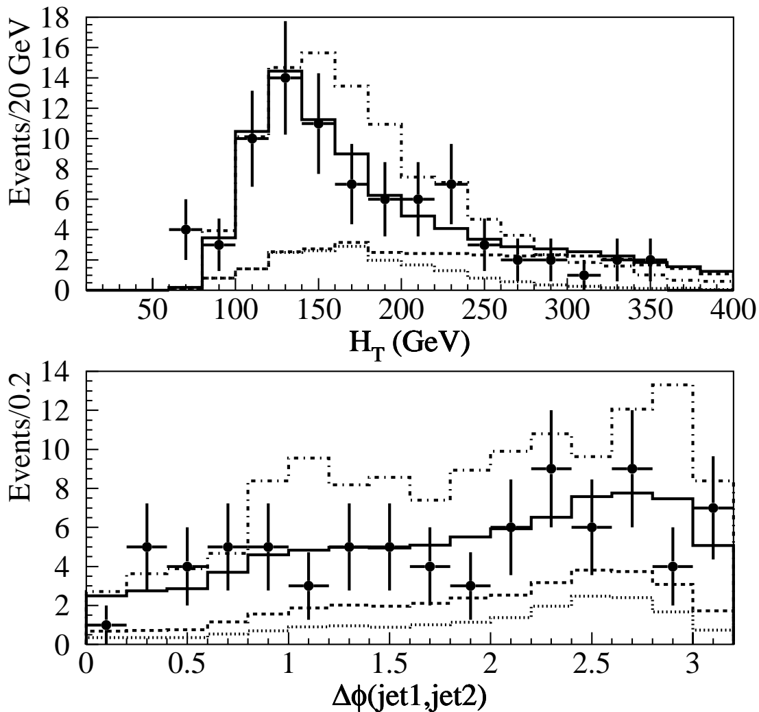
FIG. 1. Results of the two-dimensional fit to H_T and \Delta\phi(\text{jet1,jet2}) when the \tilde{t}_1 \rightarrow b\tilde{\chi}_1^+ branching ratio is 100%, m_{\tilde{t}_1} = 115 \text{ GeV}/c^2 , m_{\tilde{\chi}_1^\pm} = 90 \text{ GeV}/c^2 , and m_{\tilde{\chi}_1^0} = 40 \text{ GeV}/c^2 . The quantities H_T and \Delta\phi(\text{jet1,jet2}) are defined in the text. The points represent the data. Cumulative contributions from b\bar{b} and fake lepton events, t\bar{t} , and W^\pm \rightarrow l^\pm\nu + \text{jets} are represented by dotted, dashed and solid lines respectively. There is no significant contribution from signal. To illustrate the shape difference, a signal distribution with arbitrary normalization has been overlaid with a dot-dash line.
