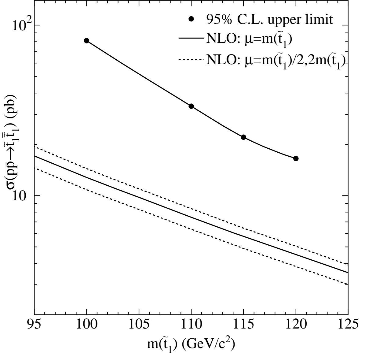
FIG. 2. The points represent the CDF 95% C.L. cross section limit as a function of \tilde{t}_1 mass when the \tilde{t}_1 \rightarrow b\tilde{\chi}_1^+ branching ratio is 100%, m_{\tilde{\chi}_1^\pm} = 90 GeV/c 2 , and m_{\tilde{\chi}_1^0} = 40 GeV/c 2 . The line without markers represents the NLO prediction for \sigma_{\tilde{t}_1 \bar{\tilde{t}}_1} using the renormalization scale \mu = m_{\tilde{t}_1} . The dashed lines represent the NLO cross section for \mu = m_{\tilde{t}_1}/2 and \mu = 2m_{\tilde{t}_1} .
