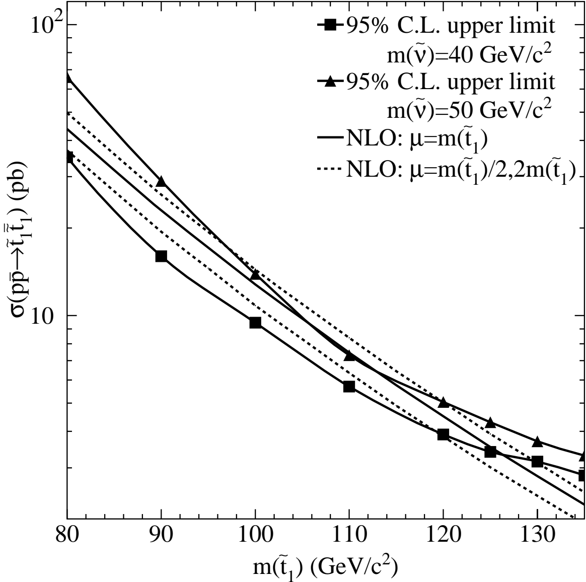
FIG. 3. CDF 95% C.L. cross section limit as a function of \tilde{t}_1 mass when the \tilde{t}_1 \rightarrow b l^+ \tilde{\nu} branching ratio is 100% and m_{\tilde{\nu}} = 40 \text{ GeV}/c^2 (squares) or 50 \text{ GeV}/c^2 (triangles). The line without markers represents the NLO prediction for \sigma_{\tilde{t}_1 \tilde{t}_1} using the renormalization scale \mu = m_{\tilde{t}_1} . The dashed lines represent the NLO cross section for \mu = m_{\tilde{t}_1}/2 and \mu = 2m_{\tilde{t}_1} .
