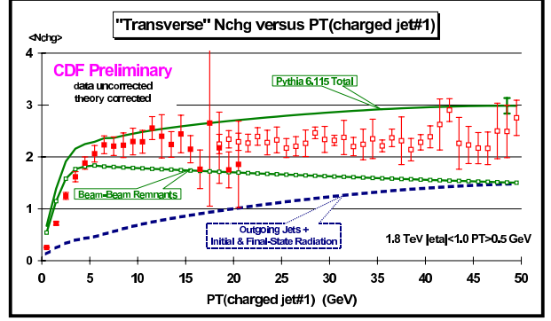
Figure 39. Data from Fig. 25 on the average number of charged particles ( p_T > 0.5 \text{ GeV} and |\eta| < 1 ) as a function of p_T(\text{jet}\#1) ( leading charged jet ) for the “transverse” region defined in Fig. 24 compared with the QCD “hard scattering” Monte-Carlo predictions of PYTHIA 6.115. The predictions of PYTHIA are divided into two categories: charged particles that arise from the break-up of the beam and target ( beam-beam remnants ), and charged particles that result from the outgoing jets plus initial and final-state radiation ( hard scattering component ). For PYTHIA, the beam-beam remnants include contributions from multiple parton scattering (see Fig. 19). The errors on the ( uncorrected ) data include both statistical and correlated systematic uncertainties. The theory curves are corrected for the track finding efficiency and have an error ( statistical plus systematic ) of around 5%.
