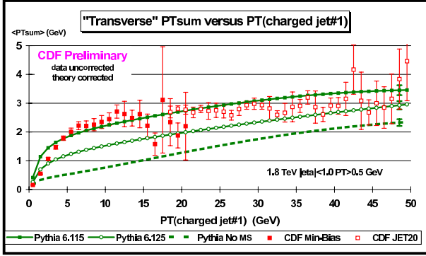
Figure 36. Data from Fig. 26 on the average scalar p_T sum of charged particles ( p_T > 0.5 GeV and |\eta| < 1 ) as a function of p_T(\text{jet}\#1) ( leading charged jet ) for the “transverse” region defined in Fig. 24 compared with the QCD “hard scattering” Monte-Carlo predictions of PYTHIA 6.115, PYTHIA 6.125, and PYTHIA with no multiple parton scattering (No MS). The errors on the ( uncorrected ) data include both statistical and correlated systematic uncertainties. The theory curves are corrected for the track finding efficiency and have an error ( statistical plus systematic ) of around 5%.
