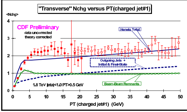
Figure 38. Data from Fig. 25 on the average number of charged particles ( p_T > 0.5 \text{ GeV} and |\eta| < 1 ) as a function of p_T(\text{jet}\#1) ( leading charged jet ) for the “transverse” region defined in Fig. 24 compared with the QCD “hard scattering” Monte-Carlo predictions of HERWIG 5.9. The predictions of HERWIG are divided into two categories: charged particles that arise from the break-up of the beam and target ( beam-beam remnants ), and charged particles that result from the outgoing jets plus initial and final-state radiation ( hard scattering component ) (see Fig. 19). The errors on the ( uncorrected ) data include both statistical and correlated systematic uncertainties. The theory curves are corrected for the track finding efficiency and have an error ( statistical plus systematic ) of around 5%.
