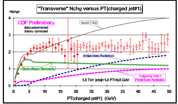
Figure 37. Data from Fig. 25 on the average number of charged particles ( p_T > 0.5 GeV and |\eta| < 1 ) as a function of p_T(\text{jet}\#1) ( leading charged jet ) for the “transverse” region defined in Fig. 24 compared with the QCD “hard scattering” Monte-Carlo predictions of ISAJET 7.32. The predictions of ISAJET are divided into three categories: charged particles that arise from the break-up of the beam and target ( beam-beam remnants ), charged particles that arise from initial-state radiation, and charged particles that result from the outgoing jets plus final-state radiation (see Fig. 19). The errors on the ( uncorrected ) data include both statistical and correlated systematic uncertainties. The theory curves are corrected for the track finding efficiency and have an error ( statistical plus systematic ) of around 5%.
