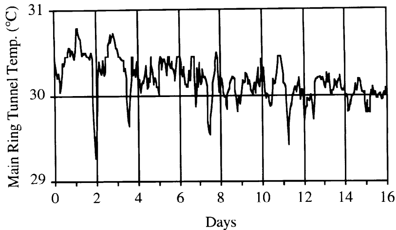
Figure 3.1.7: Measured Main Ring tunnel temperature during a typical period of operations. Note that on the second day the Main Ring was turned off for a few hour access.
