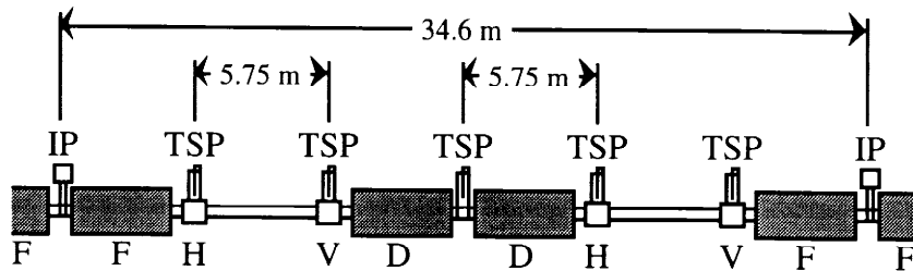
Figure 3.2.1: Sketch of the vacuum system in a normal arc cell. The horizontal (H) and vertical (V) beam position monitors have attached to them titanium sublimation pumps (TSP) in order to maintain a low average pressure and to minimize the number of welds in the tunnel.
