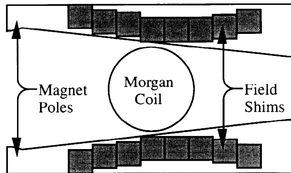
Figure 3.1.12: Sketch of the positioning of the end shim steel blocks with respect to the pole face. The position of the Morgan coil is also shown.
