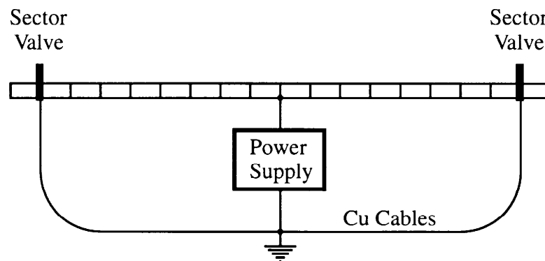
Figure 3.2.8: Sketch of the portable power supply connected across a vacuum sector used to heat the vacuum system to 150°C.
