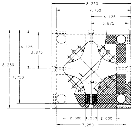
Figure 3.1.2: Quadrupole magnet profile. These magnets are composed of single bricks behind each pole.
