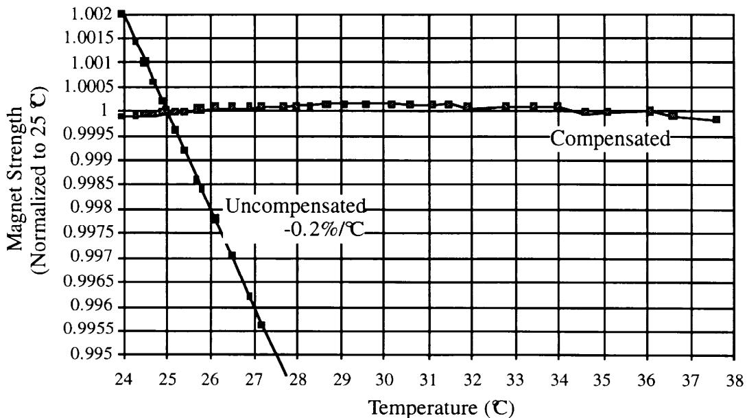
Figure 3.1.8: Field strength vs. temperature for a stability test magnet using pre-production samples from the selected vendors for compensator alloy and ferrite.
