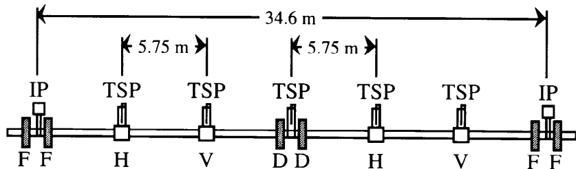
Figure 3.2.2: Sketch of the vacuum system in a normal straight section cell. Except for the fact that the quadrupoles are much shorter than the gradient magnets in the normal arc cell, nothing is different with respect to figure 3.2.1.
