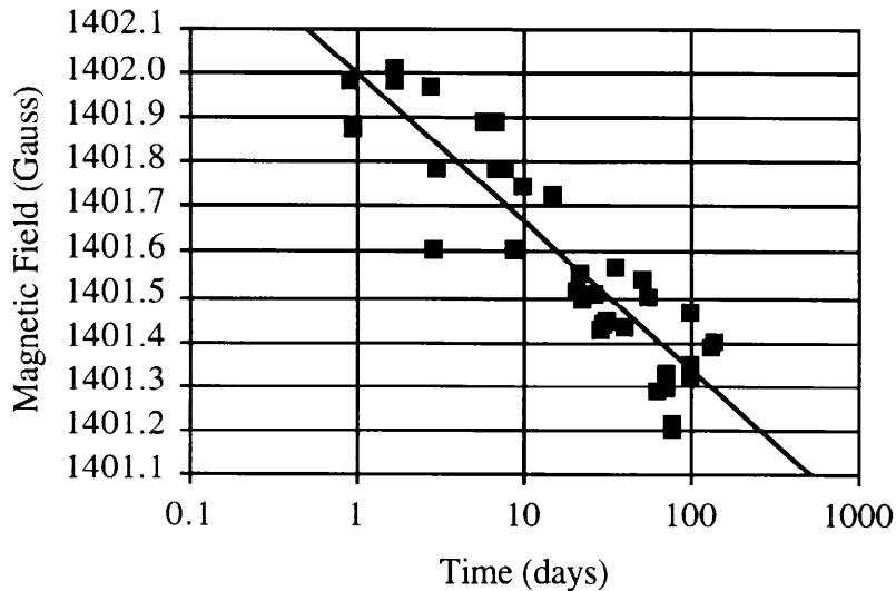
Figure 3.1.10: Field strength vs. time of a stability test magnet. This magnet was composed of bricks which were demagnetized by 5% before assembly. The line represents a log-time decay rate of 2.4 \times 10^{-4} /decade.
