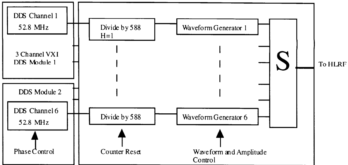
Figure 3.4.1: Block diagram of the Recycler low-level RF system.
