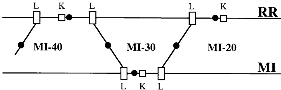
Figure 3.8.4: Sketch of the placement and number of toroids in the Main Injector and Recycler to service the instrumentation needs of the Recycler transfers. The Lambertsons (L), kickers (K), and toroids (black dots) are shown with respect to the service building the reside in.
