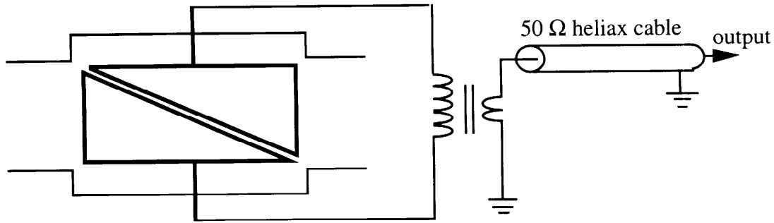
Figure 3.8.2: Sketch of the Recycler transverse Schottky electrical model. The split plate pickup provides a linear position response function. The system is resonated at 79.263 MHz ( n=882.5 ).
