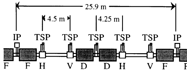
Figure 3.2.3: Sketch of the vacuum system in a dispersion suppresser cell.
