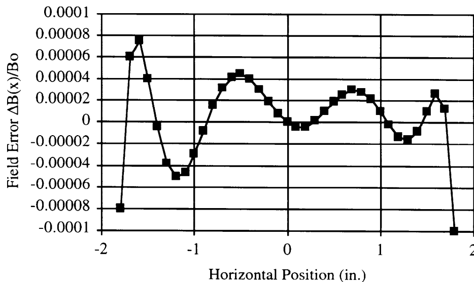
Figure 3.1.4: Design magnetic field imperfection across the horizontal aperture of a Recycler gradient magnet. Generated by Poisson, the ripple in the field is due to the finite extent of the poles and the trapezoidal approximation of the pole shape.
