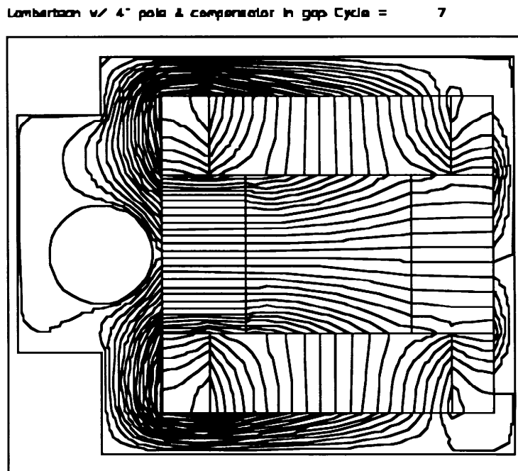
Figure 3.1.16: Permanent Lambertson magnet cross-section with POISSON field map superimposed. The field free circular region is the circulating beam aperture. The horizontal field in the extracted beam line steers the beam up or down.
