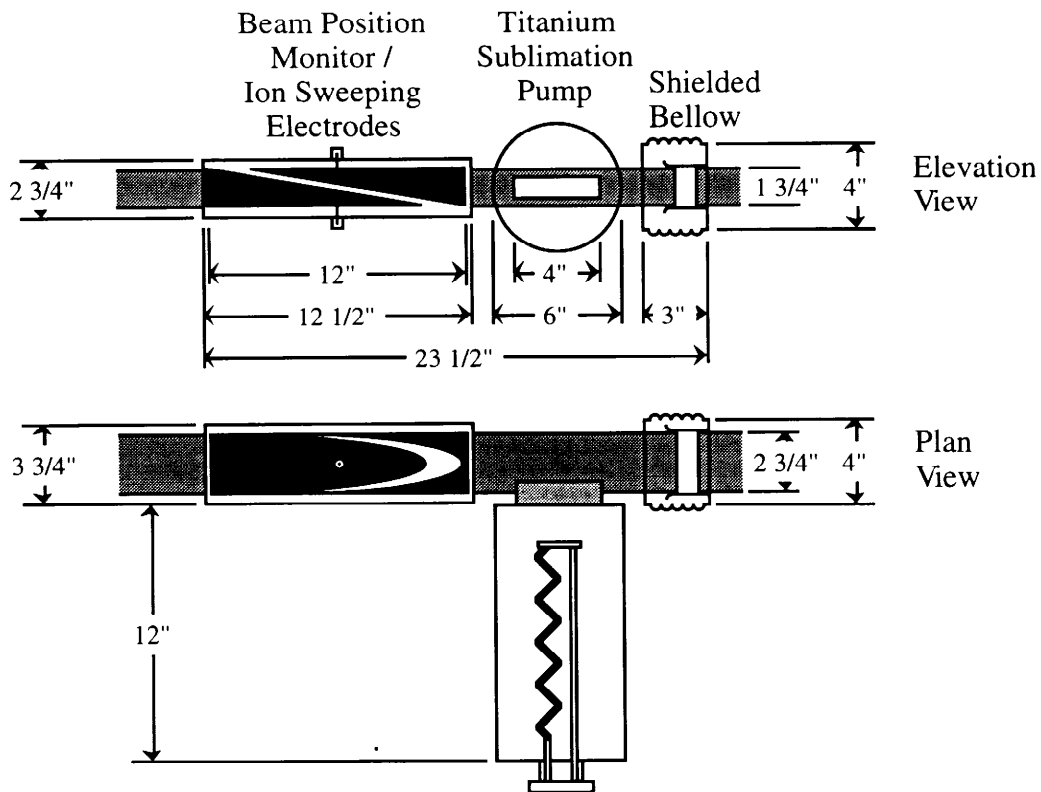
Figure 3.2.4: Elevation and plan views of the BPM assemblies which each include a TSP and shielded bellows. A vertical BPM is shown, which is on the downstream side of each half cell. The horizontal BPM, which is placed on the upstream side of each half cell, has a horizontally sensitive electrode and the entire assembly is rotated left for right.
