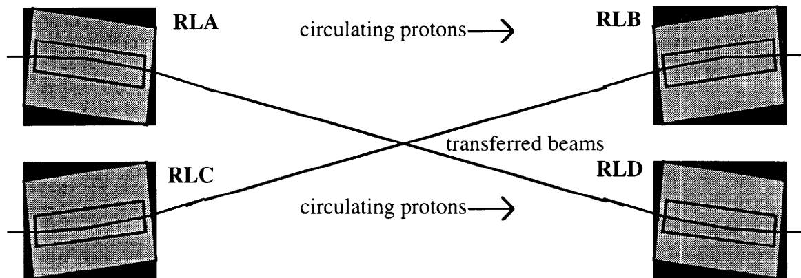
Figure 3.1.15: Lambertson construction geometries required to service all of the beam transfer needs of the Recycler.
