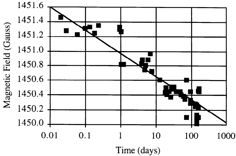
Figure 3.1.9: Field strength vs. time of a stability test magnet. Over 4 decades the data follows an expected log-time dependence. The line represents a log-time decay rate of 2.2 \times 10^{-4} /decade.
