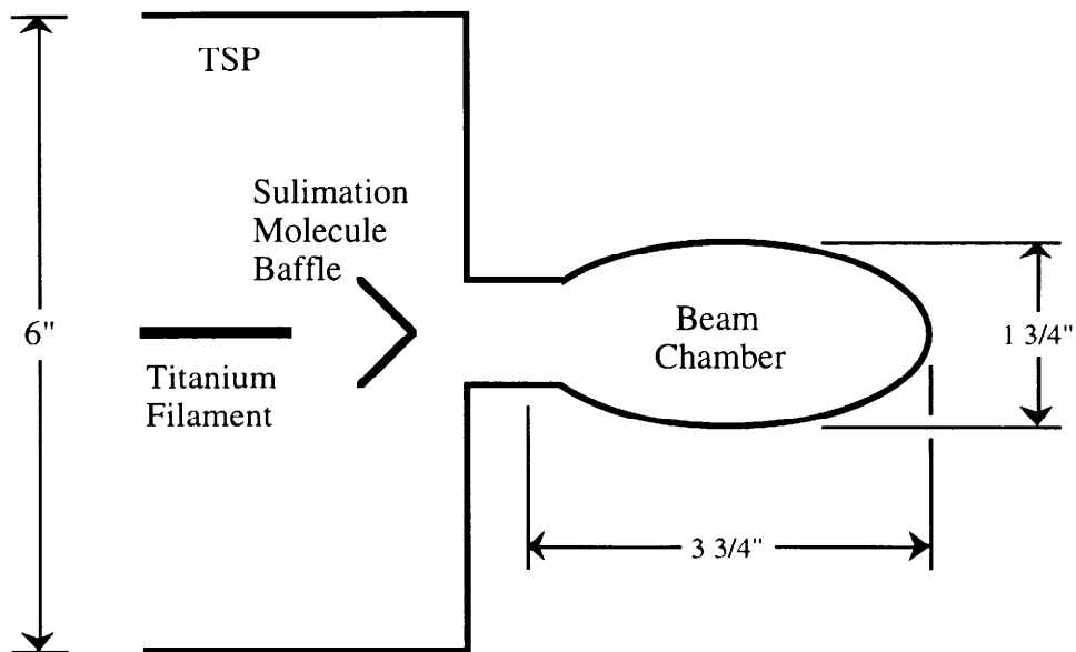
Figure 3.2.5: Beam's eye cross-section view of the TSP and its connection to the beam tube.
