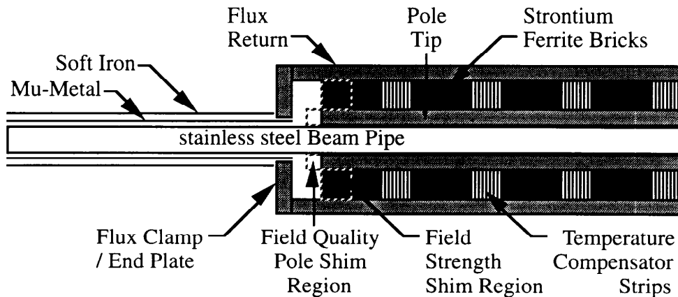
Figure 3.1.6: Side view of magnet, showing transition from magnetic shielding of naked beam pipe to magnet flux return. Also indicated are the regions at the ends of the pole tips devoted to shimming the field shape, and the ends of the ferrite bricks which are used to trim the strength of the magnet by adjusting the total amount of magnetic material.
