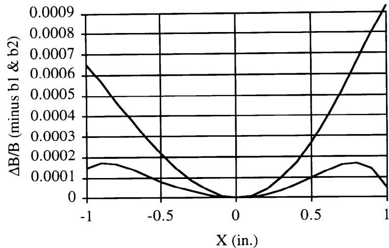
Figure 3.1.11: Short 1 m long prototype gradient magnet before (upper curve) and after (lower curve) end shims were attached to the magnet. Note that a field ripple of less than \pm 1 \times 10^{-4} was achieved.
