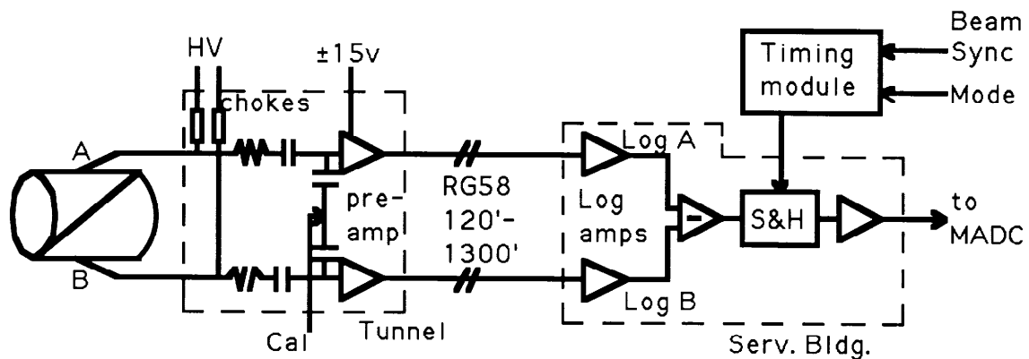
Figure 3.8.1: Block Diagram of the Recycler BPM System.
