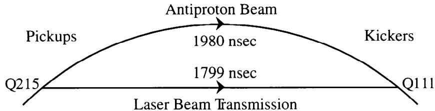
Figure 3.7.1: The chord cut by the stochastic cooling systems in order to minimize the bad mixing between the pickup and kicker.
