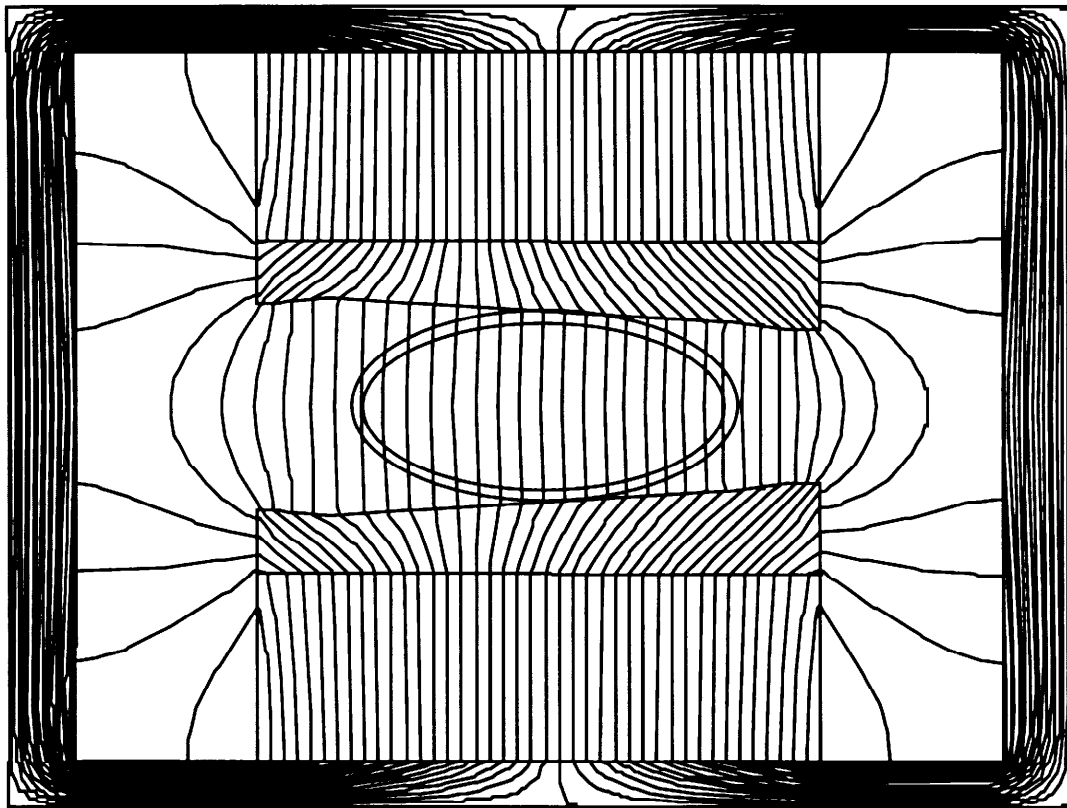
Figure 3.1.5: POISSON field map of a Recycler gradient dipole.
