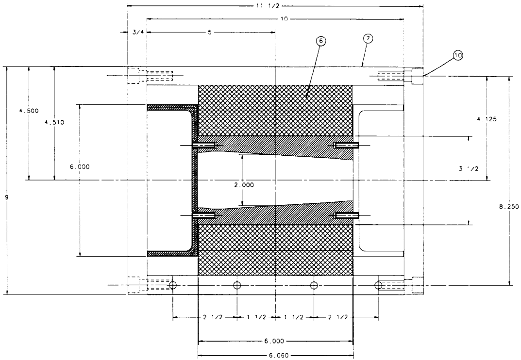
Figure 3.1.1: Gradient magnet profile. These magnets are composed of single bricks on top, on the bottom, and on each side of each pole.
