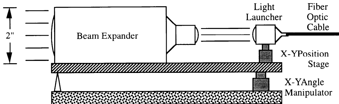
Figure 3.7.3: Sketch of the optics involved in the laser telescope. The passive optical hardware is identical on both sides of the telescope.
