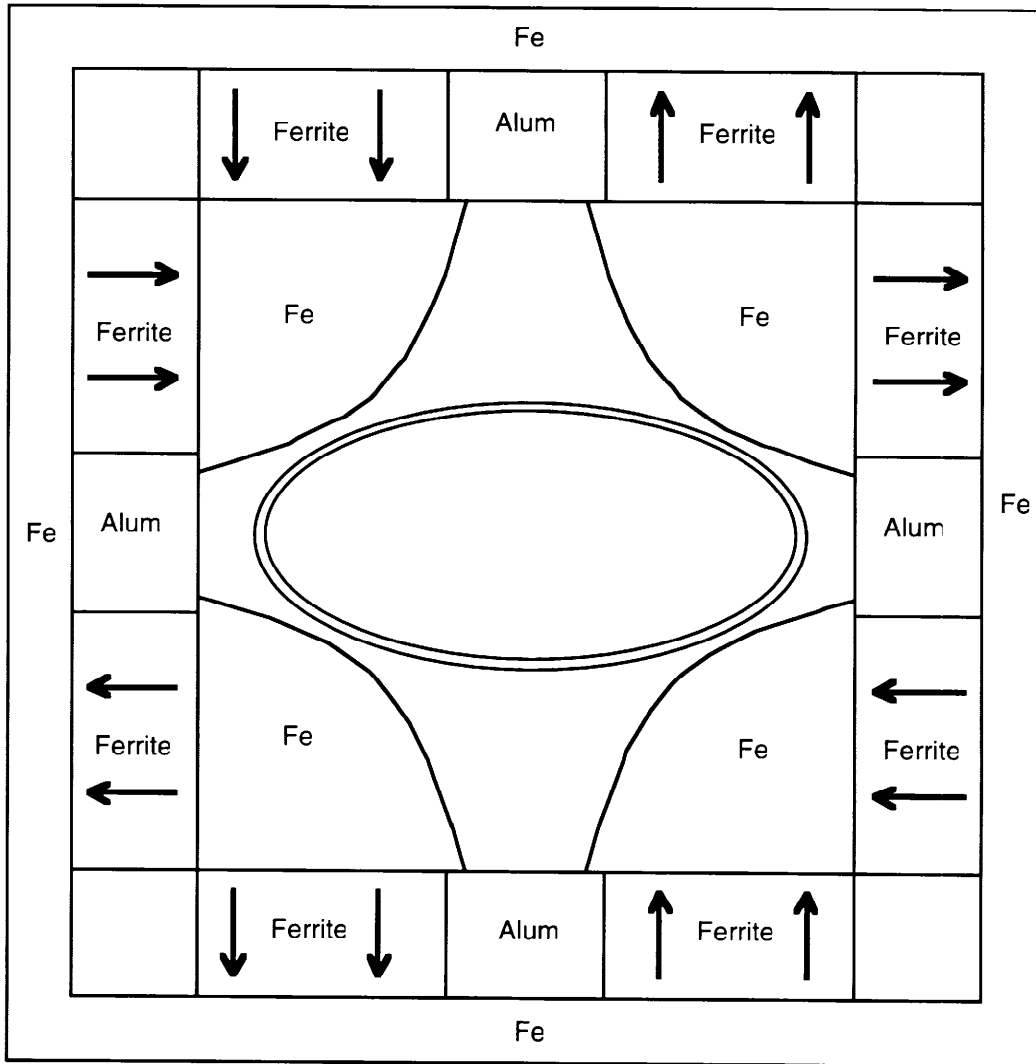
Figure 3.1.13: Cross-section of a rectangular quadrupole magnet.
