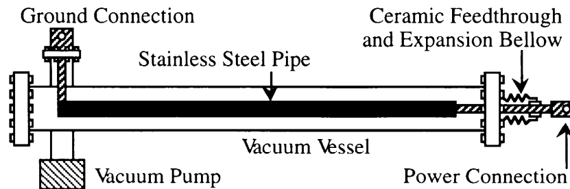
Figure 3.2.6: Sketch of the test oven which will still be used to process specialty tubing.
