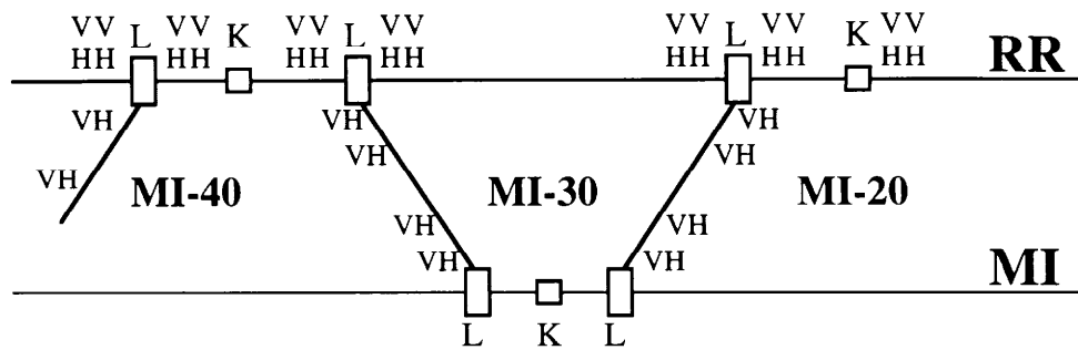
Figure 3.3.1: Locations of the horizontal (H) and vertical (V) dipole correctors in relationship with the kickers (K) and Lambertsons (L) required for the Recycler ring.
