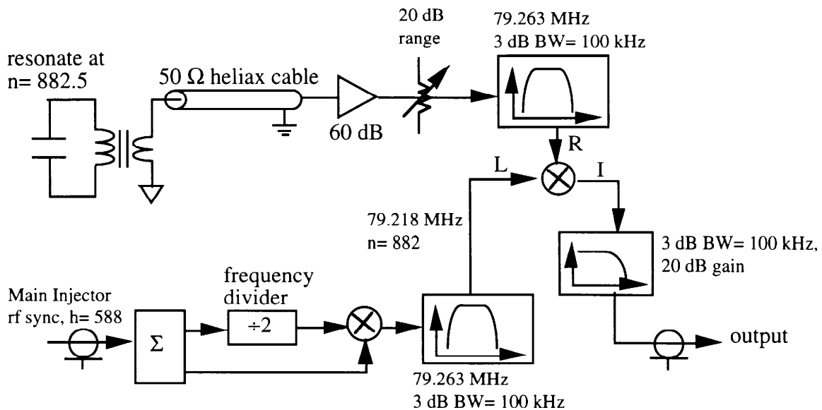
Figure 3.8.3: Sketch of the beam processing electronics which conditions the RF signal from the detector to a low frequency signal a signal analyzer can measure.
