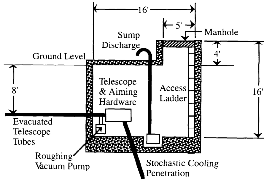
Figure 4.2.1: Sketch of one of the enclosures required at each end of the stochastic cooling signal telescope. One inexpensive model for this enclosure is a sewer access manhole constructed of round, pre-fabricated concrete components.
