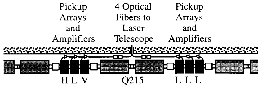
Figure 3.7.2: The relative placement of the horizontal (H), vertical (V), and momentum (L) pickup tanks with respect to the magnets. Note that the pre-amplifiers are attached to the tanks, while the laser driver for the optical fiber signal transmission are placed over the permanent magnets in order to obtain some radiation shielding from Main Injector losses.
