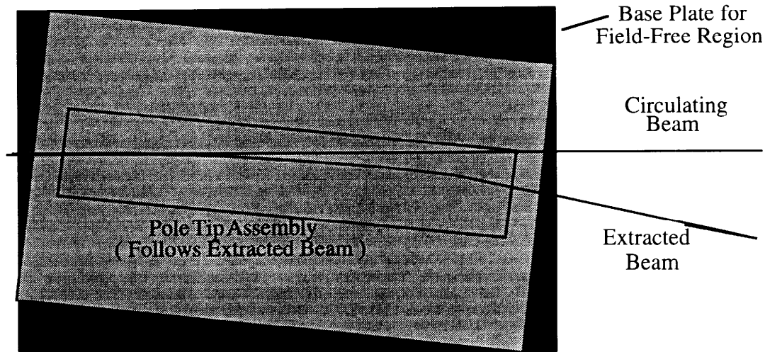
Figure 3.1.14: Side view of a Lambertson magnet showing the stored and extracted beam trajectories, and the slant in the extraction channel to minimize sagitta effects.
