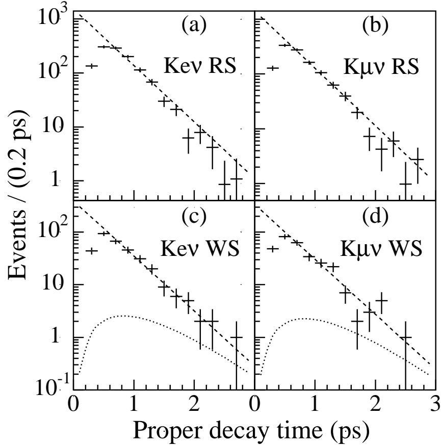
Figure 2: Dependence of RS and WS signals on proper decay time t . Crosses represent the measured decay-time distributions for (a) Ke\nu and (b) K\mu\nu background-subtracted RS signals, and for (c) Ke\nu and (d) K\mu\nu WS signal region ( Q < 0.015 \text{ GeV}/c^2 ). The dashed line in all histograms is the expected D^0 decay-time distribution uncorrected for detector acceptance, normalized to the number of events with t > 0.7 \text{ ps} (where acceptance is uniform). The dotted lines in (c) and (d) represent the expected decay-time distributions uncorrected for detector acceptance for Ke\nu and K\mu\nu mixing signals, corresponding to our 90% C.L. limit in each mode.
