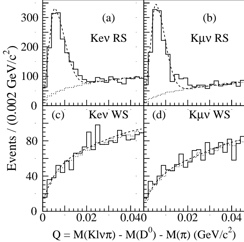
Figure 1: The Q -value distributions for (a) K_{e\nu} RS, (b) K_{\mu\nu} RS, (c) K_{e\nu} WS, and (d) K_{\mu\nu} WS candidates. The solid line histograms show the data Q -value distributions, the dashed lines are the projections of the fit in Q -value, and the dotted lines show the Q -value distribution obtained from combining a D^0 from one event and \pi from another, normalized to the number of events with Q > 0.025 \text{ GeV}/c^2 in the respective histograms.
