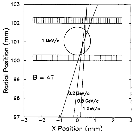
Figure 1: Pixel Micro-telescope geometry, showing trajectories of 0.2 GeV/c, 0.5 GeV/c, and 1 GeV/c tracks coming from the IP and bending in a 4 Tesla field.
