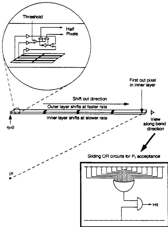
Figure 2: Pixel Micro-telescope readout scheme.
