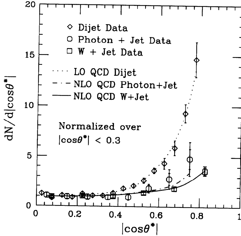
Figure 3: Selected dN/d|\cos\theta^*| for CDF W+jet data (squares), compared to previously published measurements of |\cos\theta^*| for dijet [2] and photon+jet [3] data. NLO QCD predictions are compared with the W+jet (solid curve) and the photon+jet (dashed curve) data. A LO QCD prediction (dotted curve) is compared to the dijet data. The data and theoretical predictions are all normalized to have an average value of 1 in the region |\cos\theta^*| < 0.3 .
