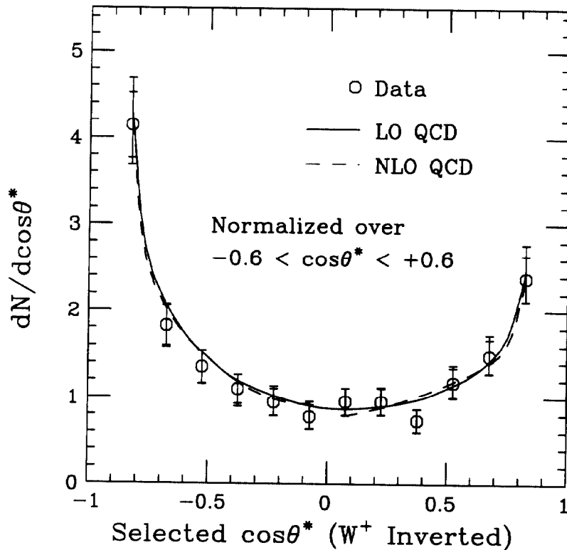
Figure 2: Selected dN/d \cos \theta^* for CDF W^+ jet data (circles), compared to a LO (solid curve) and a NLO (dashed curve) QCD prediction. The LO (NLO) theoretical prediction was generated using CTEQ1L (CTEQ1M) [18] parton distribution functions and p_T/2 for the renormalization scale. Events containing a W^+ have been inverted about zero. The asymmetry in this variable is predominantly caused by the solution selection procedure. The data and theory predictions are all normalized to have an average value of 1 in the region -0.6 < \cos \theta^* < +0.6 .
