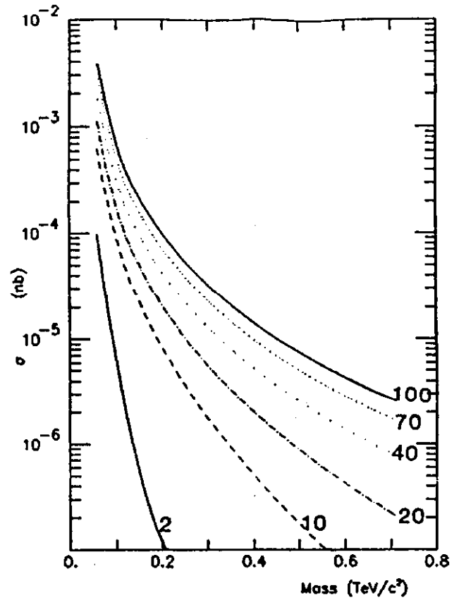
Fig. 8 Cross section for the production of H^0 H^{0'} pairs in pp collisions as a function of the H^0 mass ( H^{0'} mass assumed equal). Both H^0 and H^{0'} must satisfy |y| < 1.5 .
