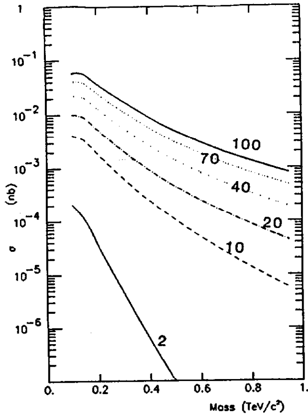
Fig. 4 Cross section for the reaction pp \rightarrow H^\pm + \text{anything} as a function of M_H , according to the parton distributions of Set 2 at \sqrt{s} = 2, 10, 20, 40, 70, and 100 TeV. Both decay products ( t\bar{b} or \bar{t}b ) must satisfy |y| < 1.5 .
