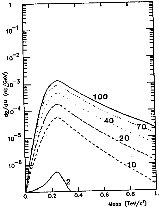
Fig. 5 Mass spectrum of t\bar{b} plus \bar{t}b plus \bar{t}b plus t\bar{b} pairs produced in proton-proton collisions, according to the parton distributions of Set 2. The rapidity of each produced quark is constrained to satisfy |y| < 1.5 .
