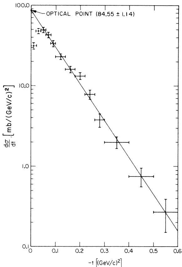
FIG. 1. Differential cross section for elastic pp scattering at 300 GeV/c. The data points shown have been corrected for the loss of proton recoils along the lens axis. The very forward points with |t| < 0.04 GeV/c suffer additional loss of short recoils at all azimuths about the beam. Those points have not been included in any fit. The smooth curve represents our best estimate of the elastic scattering differential cross section, and is a function of the form d\sigma/dt = Ae^{bt} with A = 83.82 \pm 2.06 mb/(GeV/c) 2 and b = 10.6 \pm 0.3 (GeV/c) -2 .
